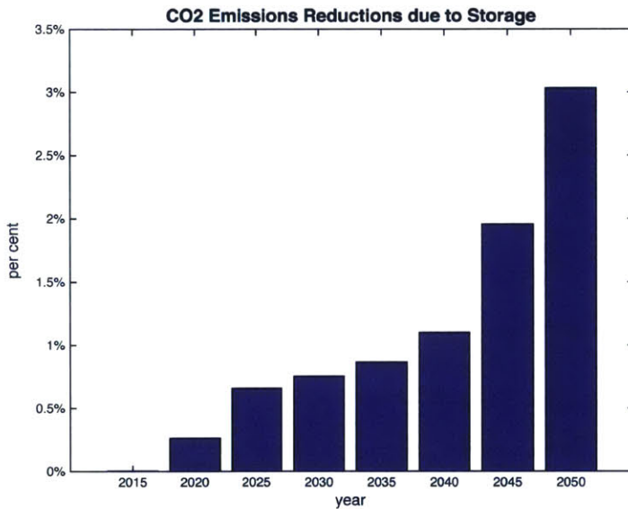
Figure 5-24: CO 2 Emissions
