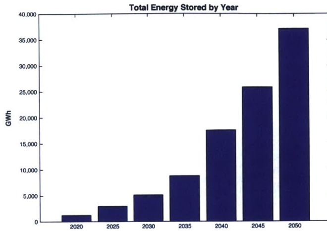
Figure 5-12: Total Energy Stored by Year
