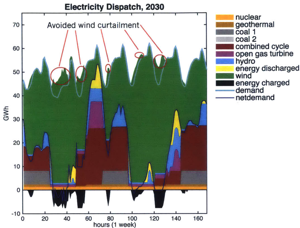
Figure 5-6: Electricity dispatch in a windy week in 2030 Source: Author-modeling results
