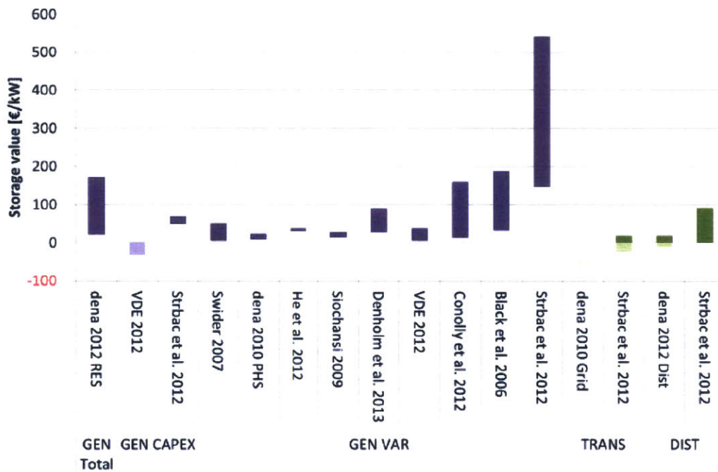
Figure 3-2: Value of Storage – System studies Source: Assessing Storage Value in Electricity Markets, Zucker et al. [202]
