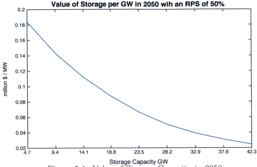
Figure 5-1: Value of Storage Capacity in 2050 Source: Author Modeling Results
