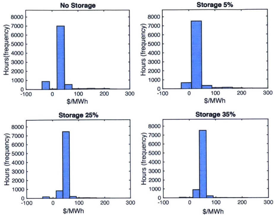
Figure 5-10: Impact of Storage on Electricity Price Volatility. Prices in 2030 at different levels of storage. Source: Author-modeling results
