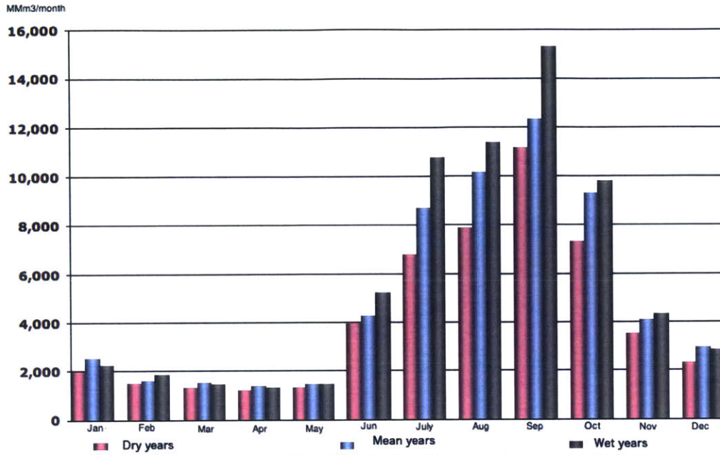
Figure 6-3: Inflows to the Big Hydro Power Facilities of Mexico (59 years of data 1952-2010)
