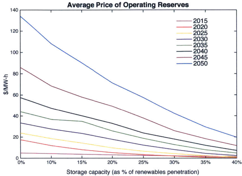
Figure 5-11: Reserves Prices Source: Author-modeling results
