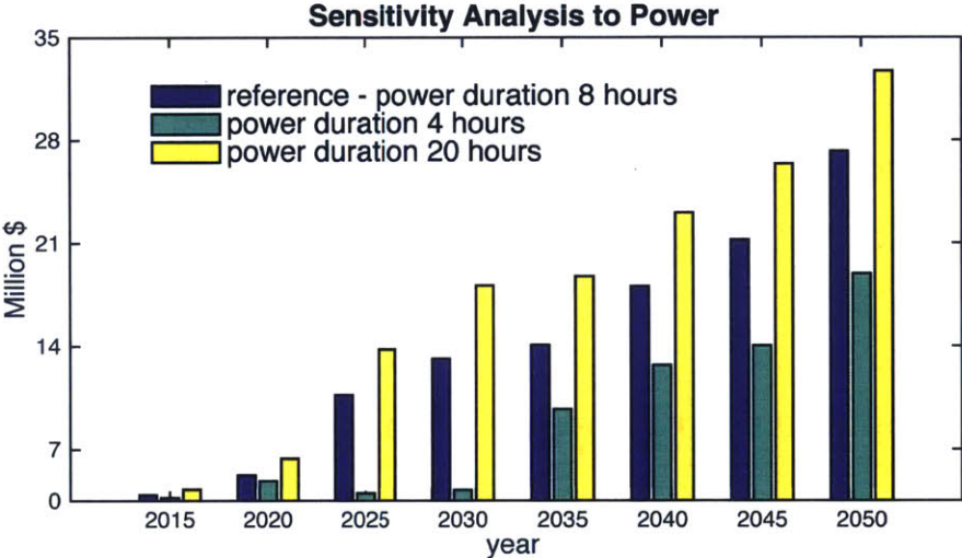
Figure 6-2: Sensitivity to Power Source: Author-modeling results
