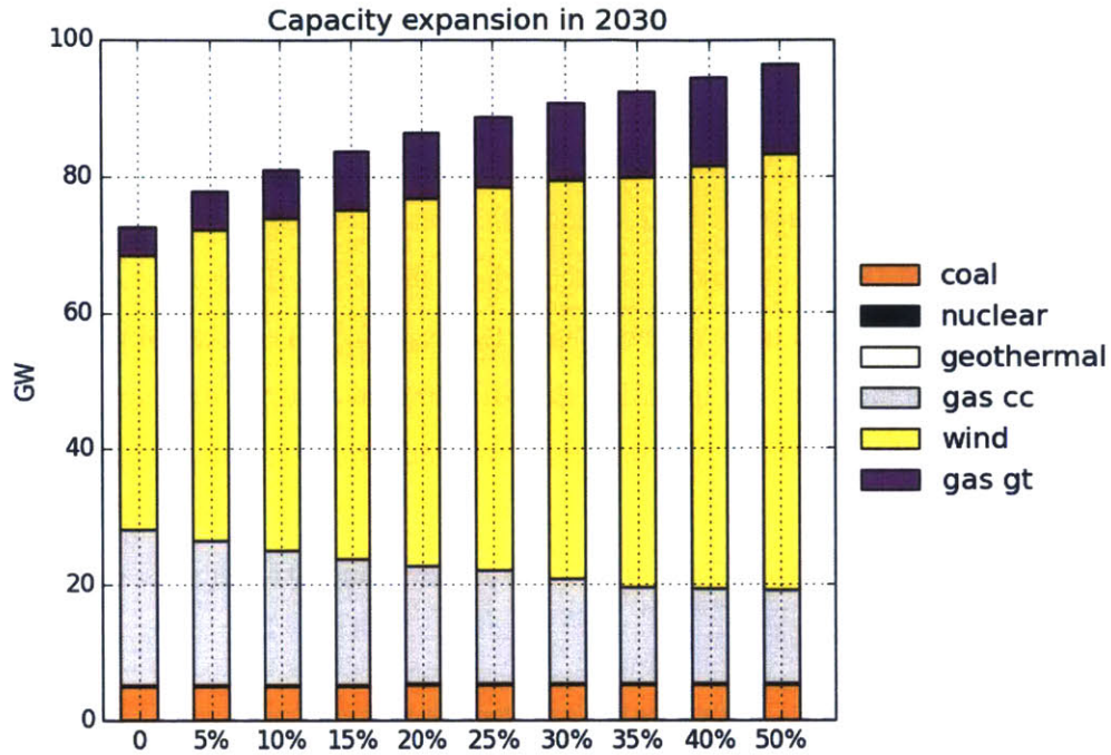
Figure 5-19: Capacity expansion in 2030 at Different Levels of Storage Capacity Source: Author-modeling results
