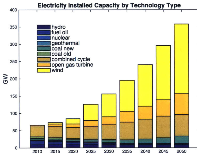
Figure 5-16: Capacity Expansion with Storage Source: Author-modeling results
