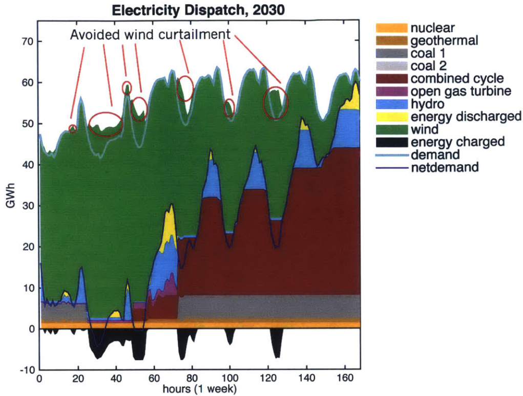
Figure 5-7: Electricity dispatch in a high wind to no wind episode in 2030 Source: Author-modeling results
