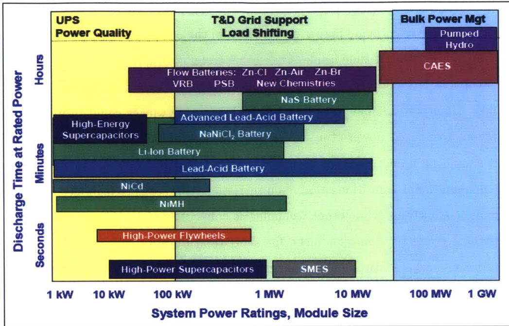
Figure 3-6: Positioning of Energy Storage Technologies
