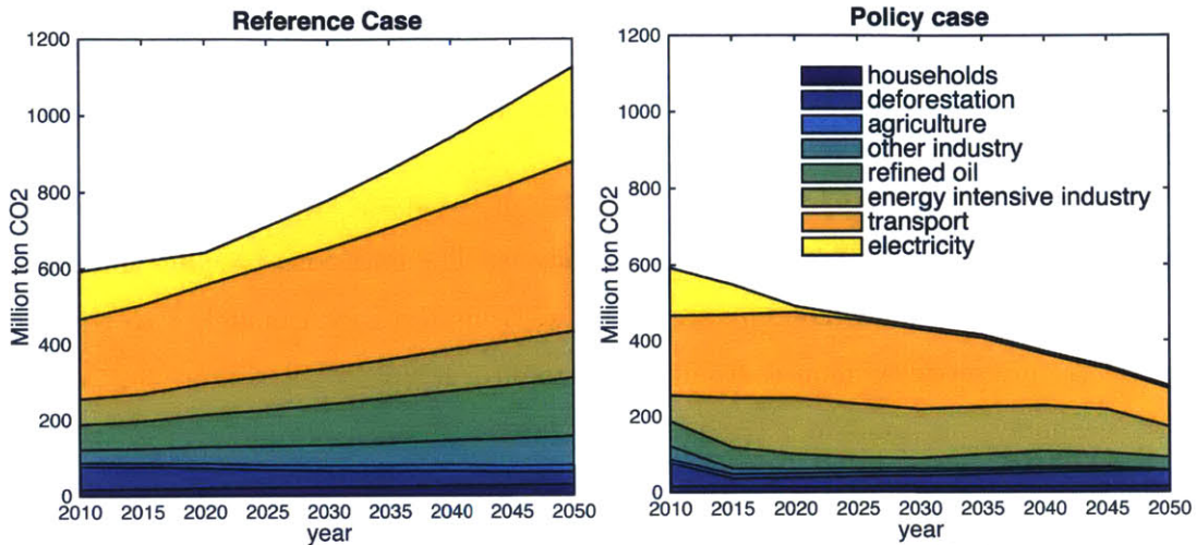
Figure 5-25: Economy-wide emissions projection 2010-2050 Source: Author-modeling results
