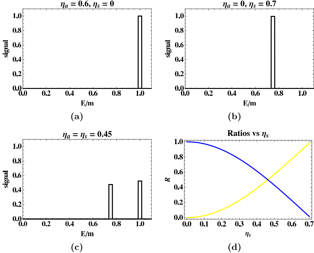
Figure 9: Injection spectrum of \phi particles in the model with Z_3 symmetry for: (a) annihilation only; (b) semi-annihilation only; (c) equal amplitudes from the two processes. The total spectrum is normalized to 1. The relative line intensities as a function of \eta_s are shown in (d), R_m^\phi (blue line) and R_{3m/4}^\phi (yellow line). The results are independent of the particle mass m_\chi .
