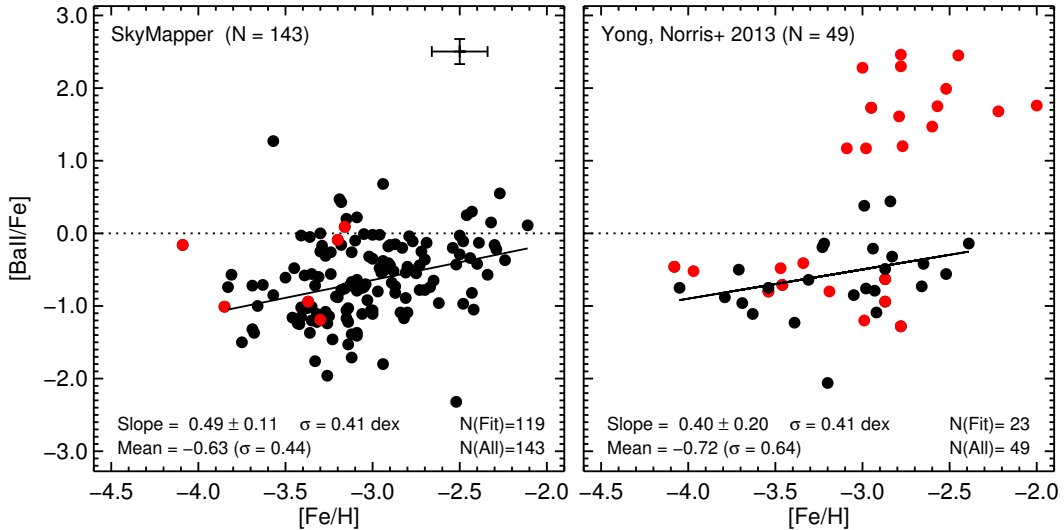
Figure 11. Same as Figure 9 but for Ba.
