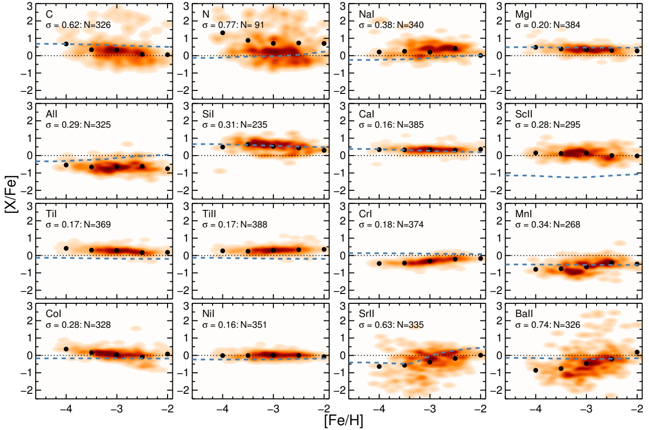
Figure 12. [X/Fe] vs. [Fe/H] for the elements from C to Ba for the current SkyMapper sample, Norris et al. (2013a), Jacobson et al. (2015) and Marino et al. (2019). (Only stars with [Fe/H] \leq -1.5 and \log g < 3 are included.) We represent the data using generalized histograms of width 0.15 dex for [Fe/H] and 0.30 dex for [X/Fe] . Average values are overplotted as filled circles and the dashed blue lines are predictions from a Galactic chemical evolution model by Kobayashi et al. (2020) updated to include stellar rotation (Kobayashi et al. in prep).
