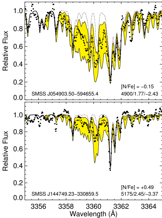
Figure 4. Same as Figure 3 but for [N/Fe] in the region 3355Å to 3365Å. The yellow shaded regions indicate \pm 0.5 dex from the best fit.
