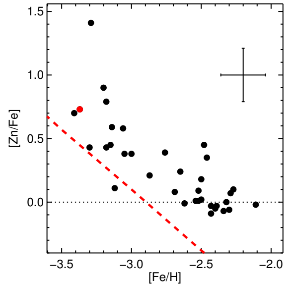
Figure 13. [Zn/Fe] vs. [Fe/H] . The red symbol is a C-rich star. The red dashed line indicates the approximate detection threshold for the 4810\text{\AA} Zn I line.
