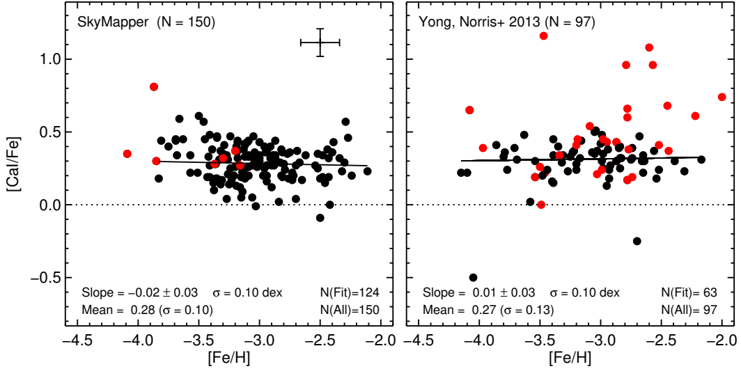
Figure 10. Same as Figure 9 but for Ca.
