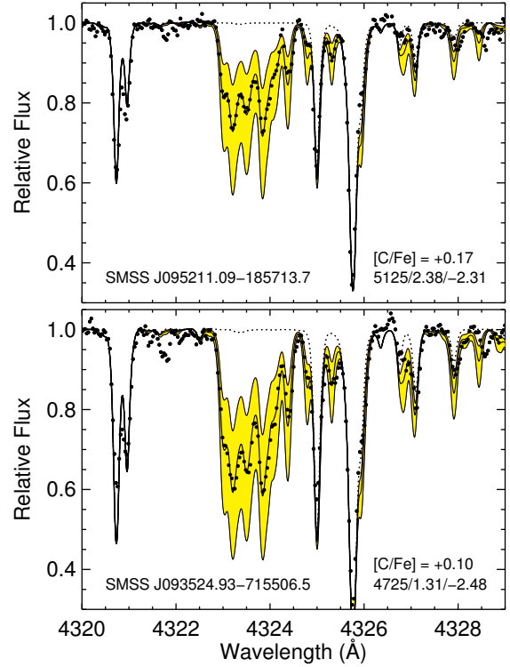
Figure 3. Comparison of observed (filled dots) and synthetic spectra in the region near 4325 Å. Synthetic spectra with no C, [\text{C}/\text{Fe}] = -9 , are shown as thin dotted lines. The best-fitting synthetic spectra are the thick black lines and the yellow shaded regions indicate \pm 0.3 dex from the best fit. The stellar parameters T_{\text{eff}}/\log g/[\text{Fe}/\text{H}] are shown.
