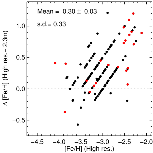
Figure 2. Comparison of the metallicities from the high-resolution Magellan spectra and the intermediate resolution ANU 2.3m spectra. The red symbols are C-rich or those flagged with G band strengths = 1. (Note that the 2.3m metallicities are quantised at the 0.25 dex level, although in some cases multiple observations were averaged.)
