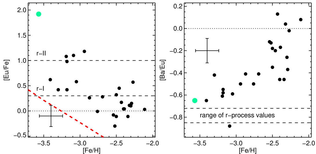
Figure 14. (Left) [\text{Eu}/\text{Fe}] vs. [\text{Fe}/\text{H}] . The aqua circle represents the neutron-capture rich star SMSS J200322.54-114203.3 and a representative error bar is included in the bottom left corner. The red dashed line indicates the approximate detection threshold for the 4129Å Eu II line. (Right) [\text{Ba}/\text{Eu}] vs. [\text{Fe}/\text{H}] . The range scaled solar r-process values ( [\text{Ba}/\text{Eu}] = -0.72 to -0.85 ) are indicated as dashed lines.
