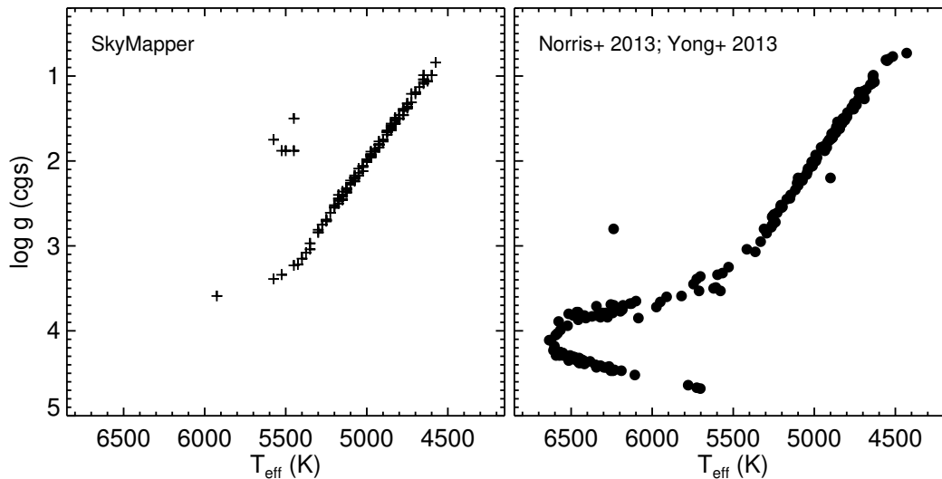
Figure 1. T_{\text{eff}} vs. \log g for the current SkyMapper sample (left) and for the Norris et al. (2013a) and Yong et al. (2013a) sample (right).
