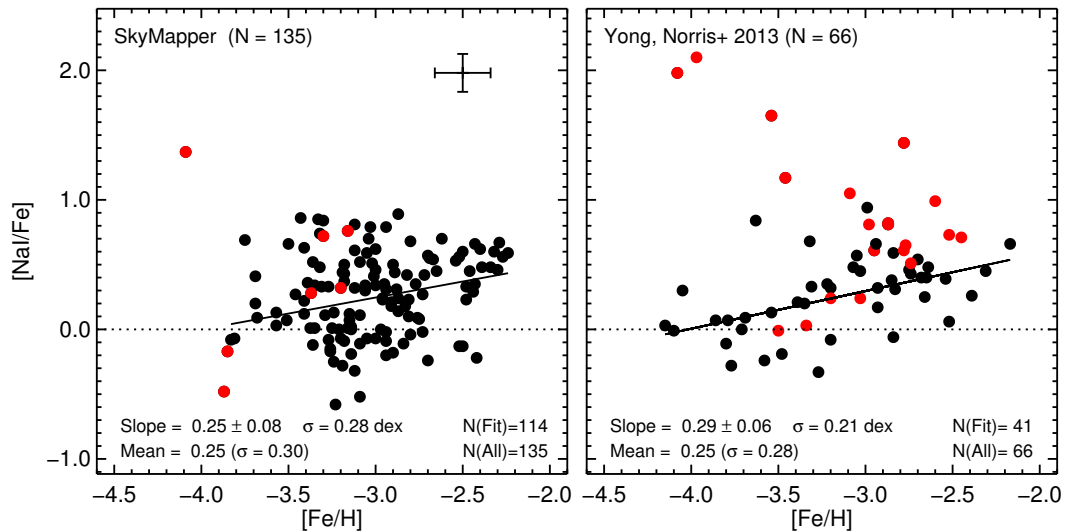
Figure 9. Same as Figure 8 but for Na. The linear fit to the data excluding C-rich stars and 2\text{-}\sigma outliers is included in each panel along with the slope, uncertainty, dispersion about the linear fit, mean, and standard deviation.
