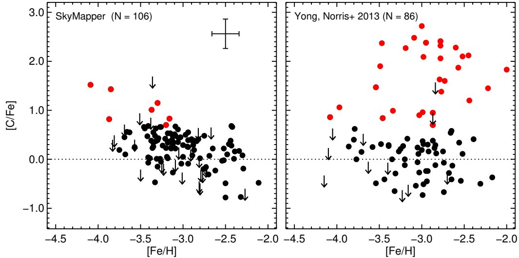
Figure 8. [C/Fe] vs. [Fe/H] for the current SkyMapper sample (left) and giants ( \log g \leq 3.0 ) from the Yong et al. (2013b) sample (right). The red symbols are C-rich objects and a representative error bar is included in the top right corner (left panel). (All C abundances are “observed”, i.e., without correction for evolutionary status.)
