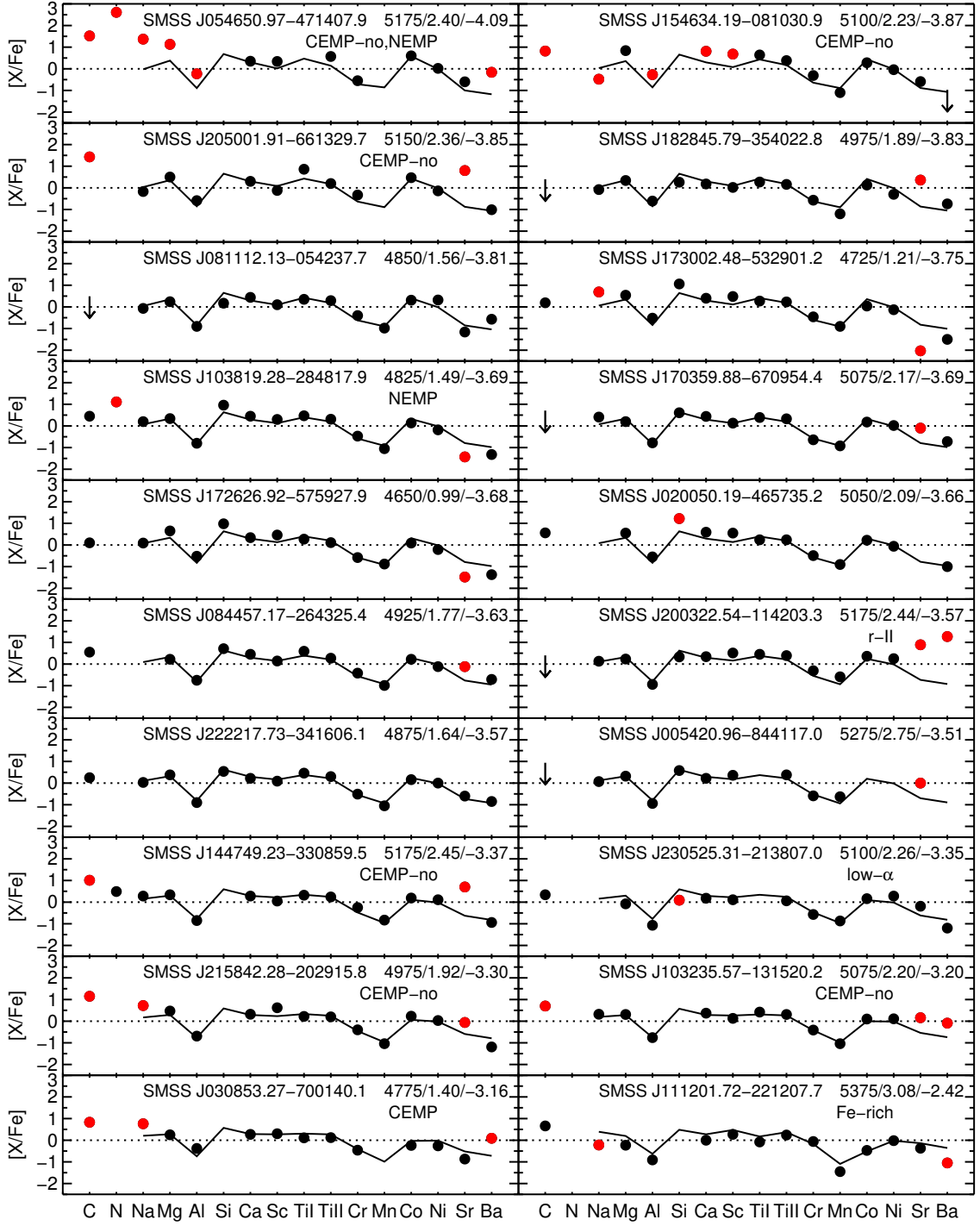
Figure 15. Abundance patterns [X/Fe] for each element for 20 program stars that are CEMP and/or with [Fe/H] < -3.5 along with representative “Fe-rich” and “low- \alpha ” objects ordered by increasing metallicity. In each panel, the solid line represents the “normal” [X/Fe] ratio at the metallicity of each program star. The model parameters ( T_{\text{eff}} , \log g , [Fe/H] ) are included in each panel. Red circles indicate when [C, N/Fe] \geq +0.7 dex, or when [X/Fe] differs from the solid line by more than 0.5 dex.
