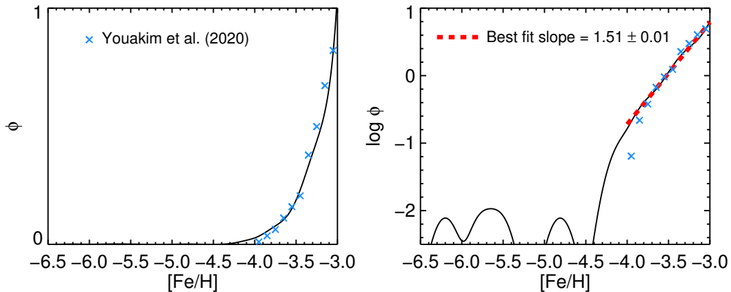
Figure 7. The metallicity distribution function in generalised histogram form (black lines) using linear (left) and logarithmic (right) scales for the combined sample (this study including SMSS J160540.18-144323.1 from Nordlander et al. (2019) plus Norris et al. 2013a). In the right panel, we fit the slope between -4 \leq [\text{Fe}/\text{H}] \leq -3 . In both panels, we overplot data from Youakim et al. (2020) (corrected with their Gaussian mixture model and colour cuts and normalised at [\text{Fe}/\text{H}] = -3.05 ) as blue crosses.
