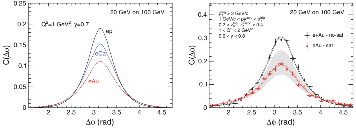
Fig. 49. Left: a saturation model prediction of the coincidence signal versus azimuthal angle difference \Delta\phi between two hadrons in e + p , e + \text{Ca} , and e + \text{A} collisions [192–194]. Right: A comparison of saturation model prediction for e + \text{A} collisions with calculations from conventional non-saturated model. Statistical error bars correspond to 1 \text{ fb}^{-1}/\text{A} integrated luminosity.
