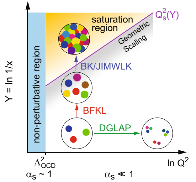
Fig. 39. The map of high energy QCD in the (Q^2, Y = \ln 1/x) plane.
