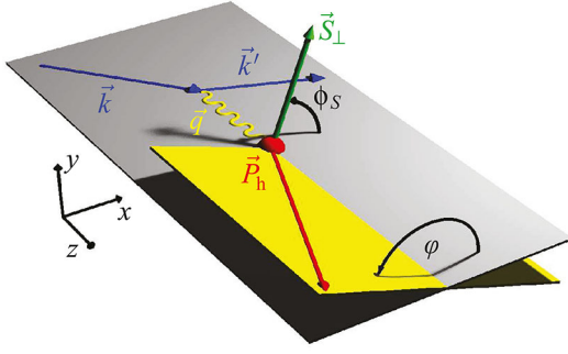
Fig. 15. Semi-inclusive hadron production in DIS processes: e + N \rightarrow e' + h + X , in the target rest frame. \vec{P}_{hT} and \vec{S}_\perp are the transverse components of \vec{P}_h and \vec{S} with respect to the virtual photon momentum \vec{q} = \vec{k} - \vec{k}' .
