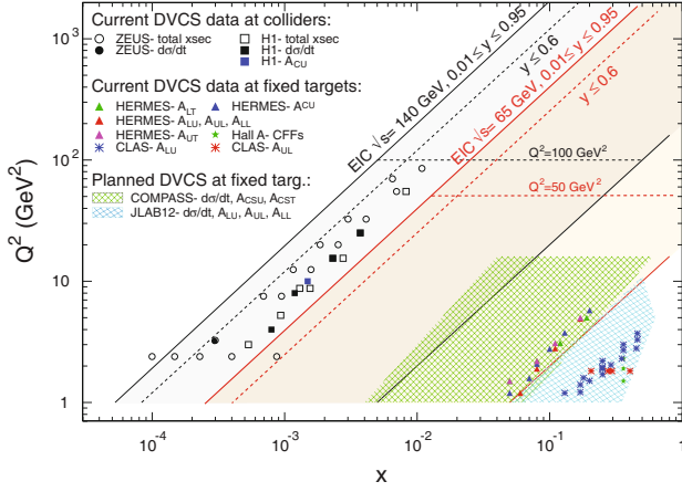
Fig. 24. An overview of existing and planned measurements of DVCS in the (x, Q^2) -plane.
