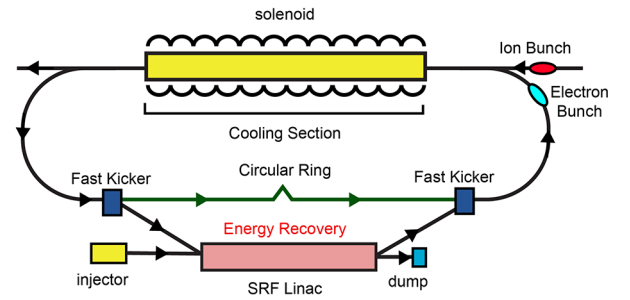
Fig. 88. Schematic of electron cooling for the JLEIC.
