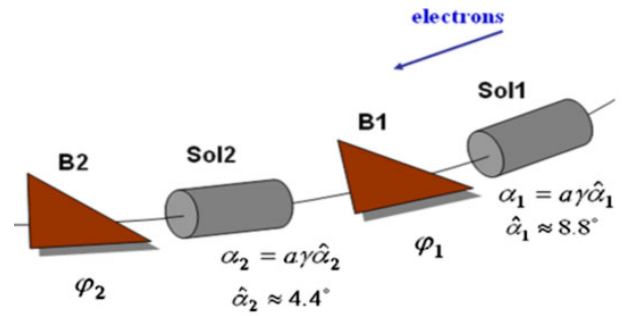
Fig. 87. Schematic drawing of a universal spin rotator consisting of two sets of arc dipoles (B1 and B2) and two solenoids (Sol1 and Sol2).
