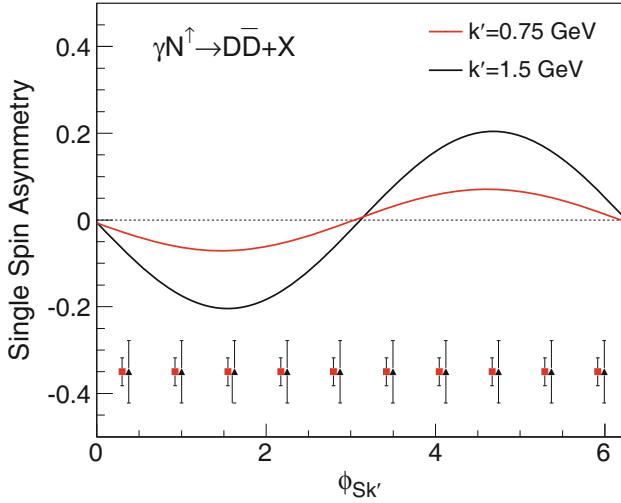
Fig. 22. The single-transverse-spin asymmetry for \gamma^* N^\uparrow \rightarrow D^0 \bar{D}^0 + X , where \phi is the azimuthal angle between the total transverse momentum k'_\perp of the D\bar{D} pair and the transverse polarization vector S_\perp of the nucleon. The asymmetries and the experimental projections are calculated for two different k'_\perp = 0.75, 1.5 GeV as examples. The kinematics are specified by \langle W \rangle = 60 GeV, \langle Q^2 \rangle = 4 GeV 2 .
