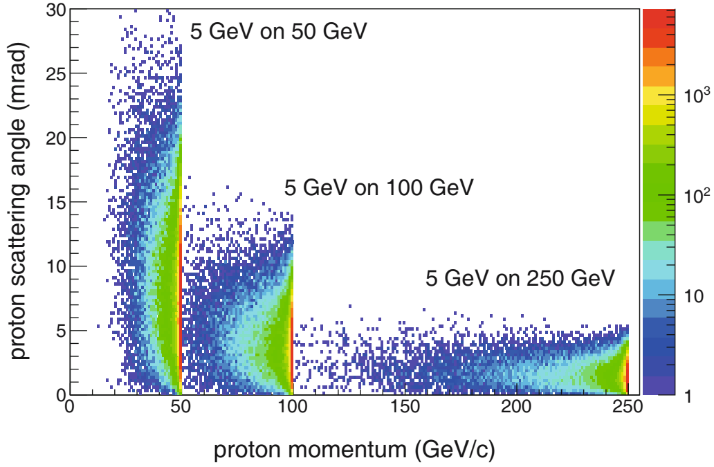
Fig. 93. The scattered proton momentum vs. scattering angle in the laboratory frames for DVCS events with different beam energy combinations. The following cuts have been applied: 1 \text{ GeV}^2 < Q^2 < 100 \text{ GeV}^2 , 0.00001 < x < 0.7 and 0 < t < 2 \text{ GeV}^2 . The angle of the recoiling hadronic system is directly and inversely correlated with the proton energy. It thus decreases with increasing proton energy.
