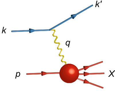
Fig. 7. A schematic diagram of the Deep Inelastic Scattering (DIS) process.
