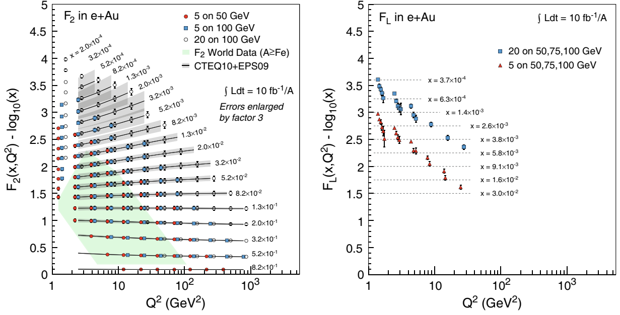
Fig. 46. The structure functions F_2 (left) and F_L (right) as functions of Q^2 for various x values in e + \text{Au} collisions at an EIC generated by using PYTHIA with EPS09 nuclear PDFs [176]. F_2 and F_L are offset by \log_{10}(x) for clarity. Measurements and corresponding errors at different energies (indicated in the panels) are presented and illustrate the respective kinematic reach. Data points from different energies at the same Q^2 are slightly offset along the abscissa for visibility where necessary. Statistical errors for F_2 and F_L are based on 10 \text{ fb}^{-1}/\text{A} integrated luminosity for the sum of all measurements at all indicated energies. Both for F_2 and F_L we assumed a 3% systematic uncertainty and added it to the statistical errors in quadrature; for F_2 the combined errors are scaled up by a factor of 3 to make them visible. For F_2 , we also depict the curves and respective uncertainty bands from the EPS09 parameterization of the nuclear parton distribution functions [176, 190]. The green shaded area indicates the (Q^2, x) range of existing measurements for nuclei larger than iron, demonstrating the kinematic reach of an EIC.
