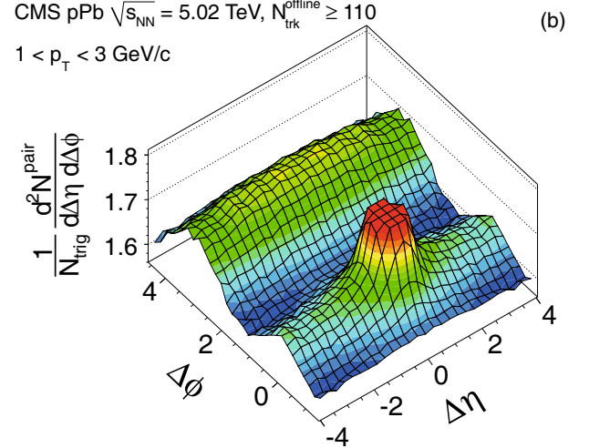
Fig. 64. The two-particle correlation function in high-multiplicity p + \text{Pb} collisions as a function of \Delta\phi and \Delta\eta reported by the CMS Collaboration [254]. The “ridge” structure is seen as a correlation near \Delta\phi = 0 stretching over many units of rapidity \Delta\eta .
