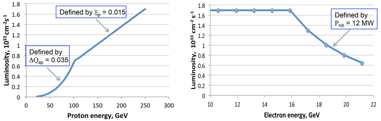
Fig. 77. eRHIC luminosity as a function of electron and proton beam energy. The left plot shows the luminosity dependence on proton energy at E_e = 15.9 \text{ GeV} . The right plot presents the luminosity as a function of electron energy at E_p = 250 \text{ GeV} .
