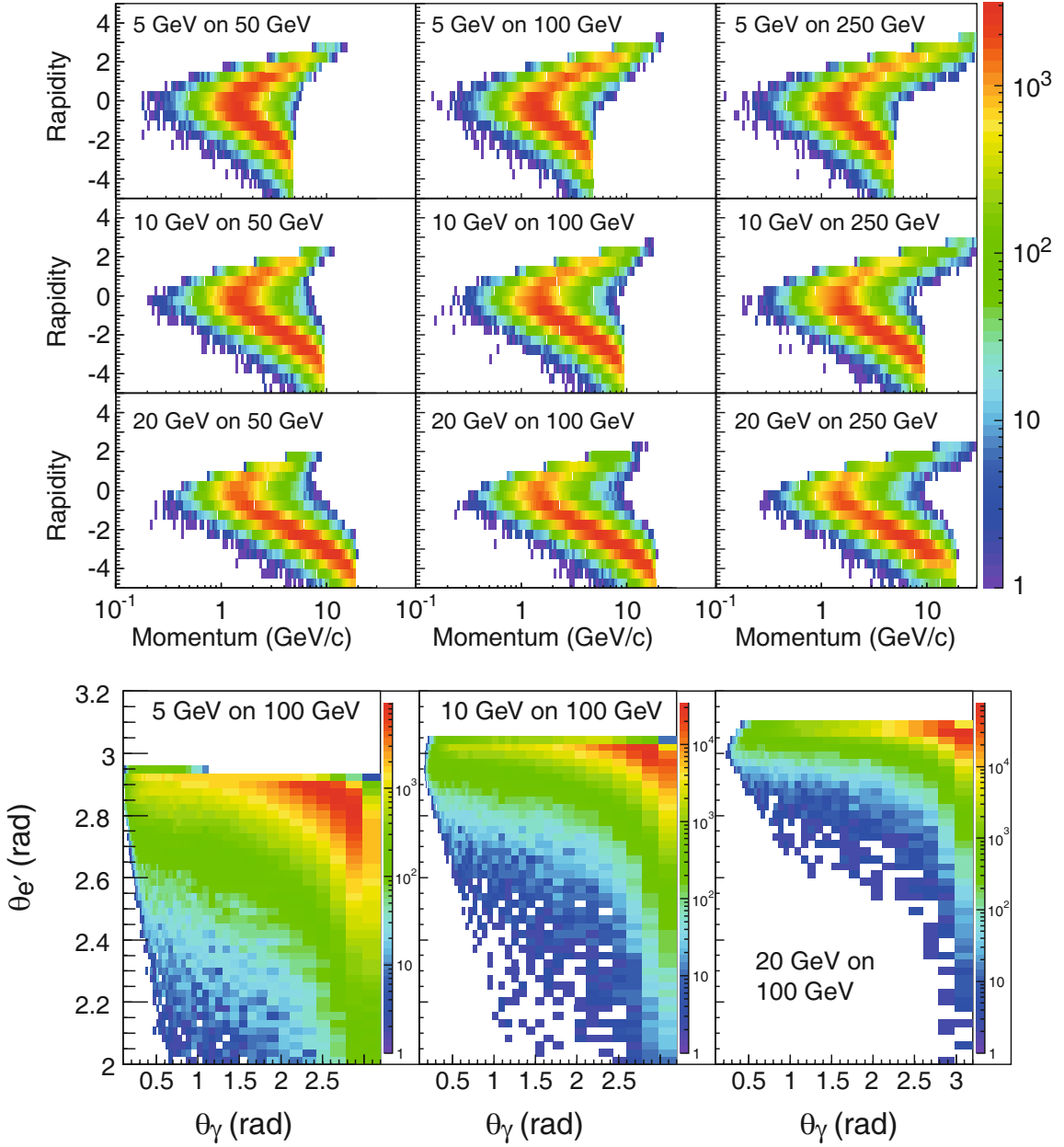
Fig. 92. The energy vs. rapidity in the laboratory frame for photons from DVCS for different center-of-mass energies (top) and the correlation between the scattering angle of the DVCS photon and the scattered lepton for three different center-of-mass energies. The following cuts have been applied: Q^2 > 1.0 \text{ GeV}^2 , 0.01 < y < 0.95 , E_\gamma > 1 \text{ GeV} and -5 < \text{rapidity} < 5 .
