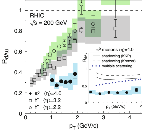
Fig. 61. The nuclear modification factor ( R_{dAu} ) versus p_T for minimum bias d + Au collisions measured at RHIC. The solid circles are for \pi^0 mesons [237], the open circles and boxes are for negative hadrons [235]. The error bars are statistical, the shaded boxes are point-to-point systematic errors. (Inset) R_{dAu} for \pi^0 mesons compared with pQCD calculations based on collinear factorization. Note that none of the curves can describe the data.
