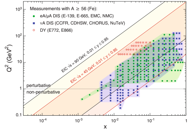
Fig. 32. The kinematic acceptance in x and Q^2 of completed lepton-nucleus (DIS) and Drell-Yan (DY) experiments (all fixed target) compared to two EIC energy options. The acceptance bands for the EIC are defined by Q^2 = xys with 0.01 \leq y \leq 0.95 and values of s shown.
