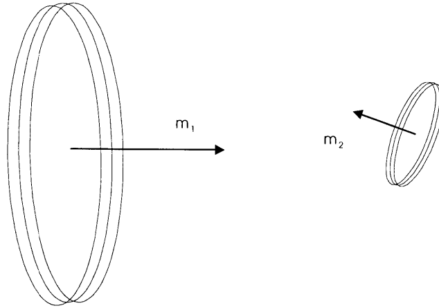
Figure 71. Diagram illustrating the dipole model for a magnetically-coupled tag system. The mutual inductance between two coils, in the far-approximation, is proportional to m_1 \cdot m_2 , where m = niA .
