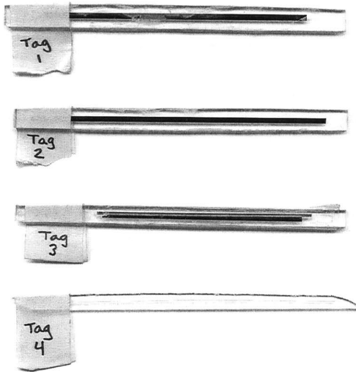
Figure 58. Photograph of VCB magnetic strips mounted on Plexiglas employed for the time-domain measurements. The strip on the bottom (#4) is an amorphous wire sample made by Unitika in Japan.
