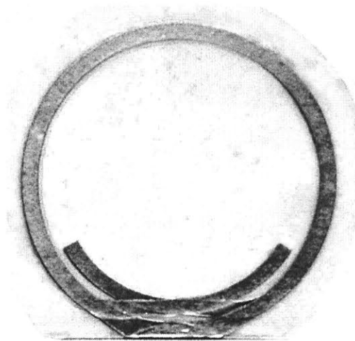
Figure 93. Photograph of sample single resonance tag used in the parameter study. The tag shown has \Theta = 420^\circ with diameter = 2.5 inches.
