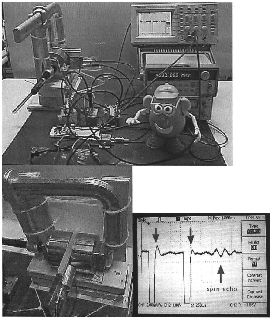
Figure 128. Photographs of table-top NMR instrumentation as well as oscilloscope signal.
