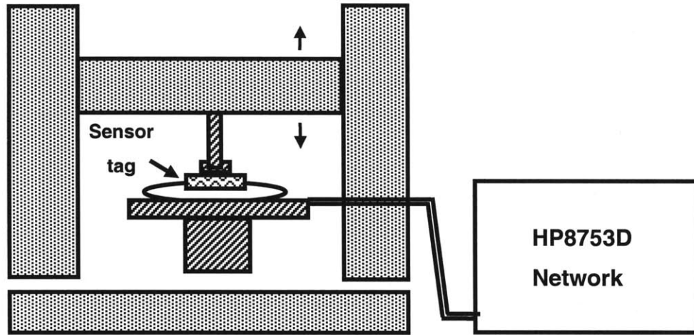
Figure 111. Schematic diagram of the test apparatus for testing the force sensor.
