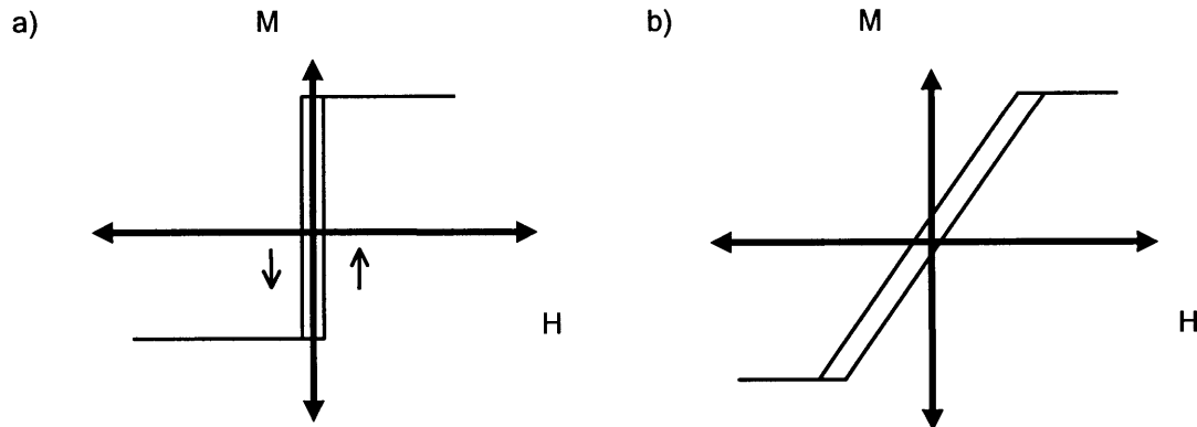
Figure 38. a) M vs H for H applied along the easy magnetic axis b) M vs H for H applied perpendicular to the magnetic easy axis
