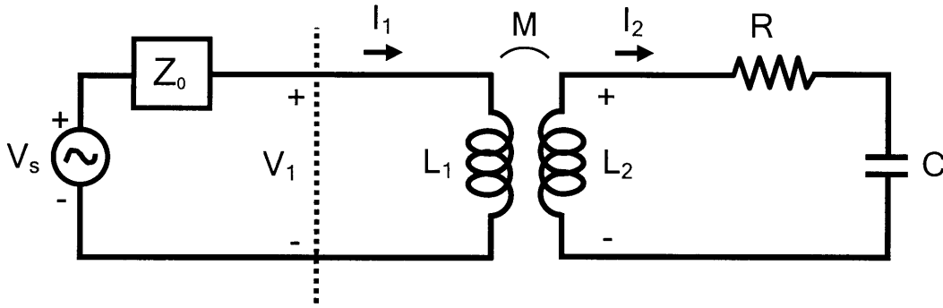
Figure 74. Circuit model for a resonator inductively coupled to a reader.
