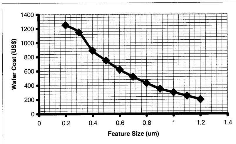
Figure 6. Wafer cost and feature size data for the past 20 years [Maly].
