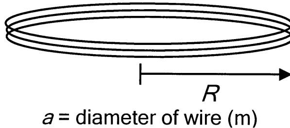
Figure 66. Diagram showing relevant coil dimensions for inductance calculation.
