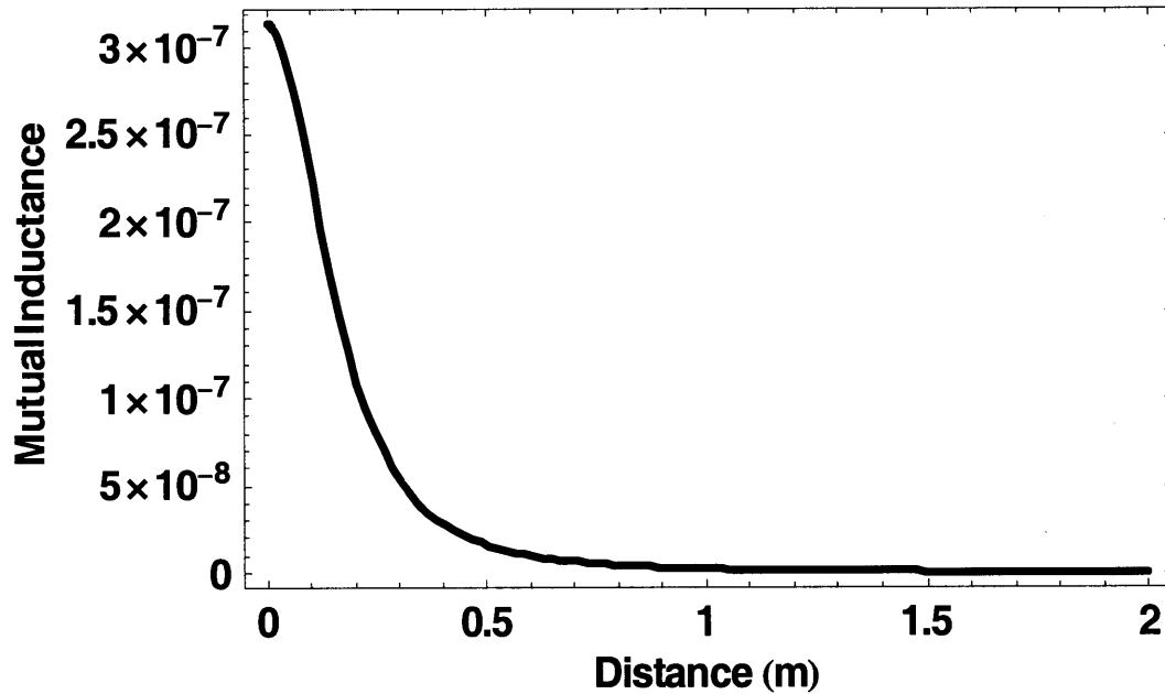
Figure 73. Sample plot of mutual inductance as a function of distance between a typical EAS tag and reader, with tag diameter = 2cm and reader coil diameter = 40cm.
