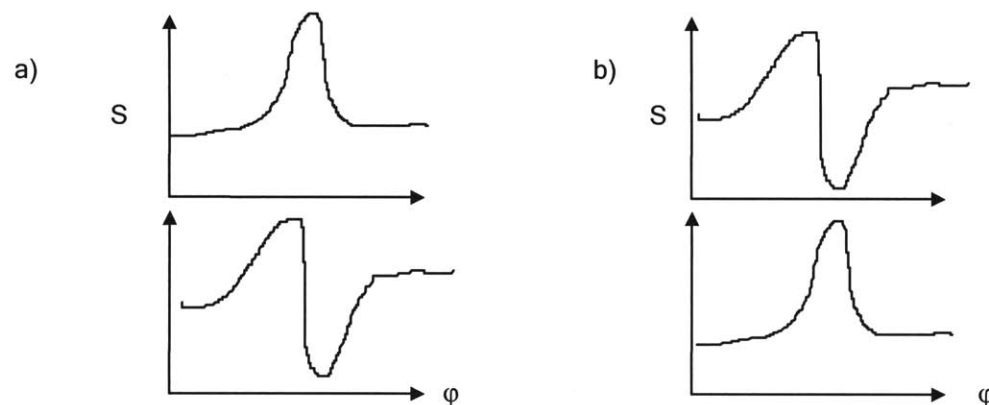
Figure 18. Amplitude S and phase \phi as a function of frequency for a) an LC resonator and b) a magnetoelastic resonator.
