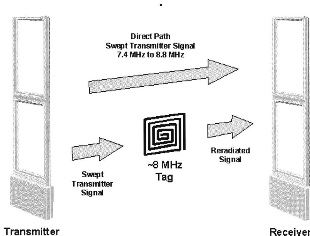
Figure 70. Illustration of reader configuration employed in a typical 8 MHz EAS system.
