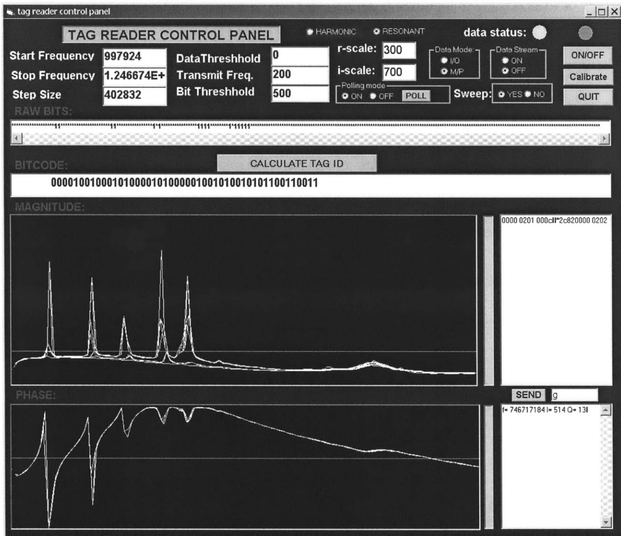
Figure 105. PC Windows interface implemented in Visual Basic showing spectra for a multi-resonant tags and also displaying the raw frequency bin data bits as well as a compact “bitcode” representation
