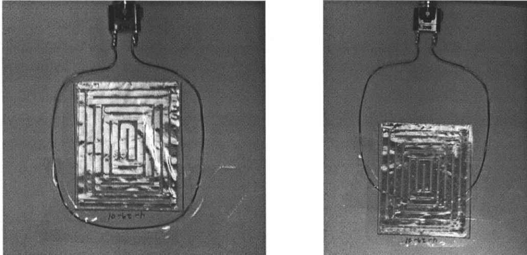
Figure 87. Photograph of loop antenna used as test probe. The photo on the left shows the standard measurement geometry. The photograph on the right depicts a misaligned tag which gives rise to additional parasitic resonances.
