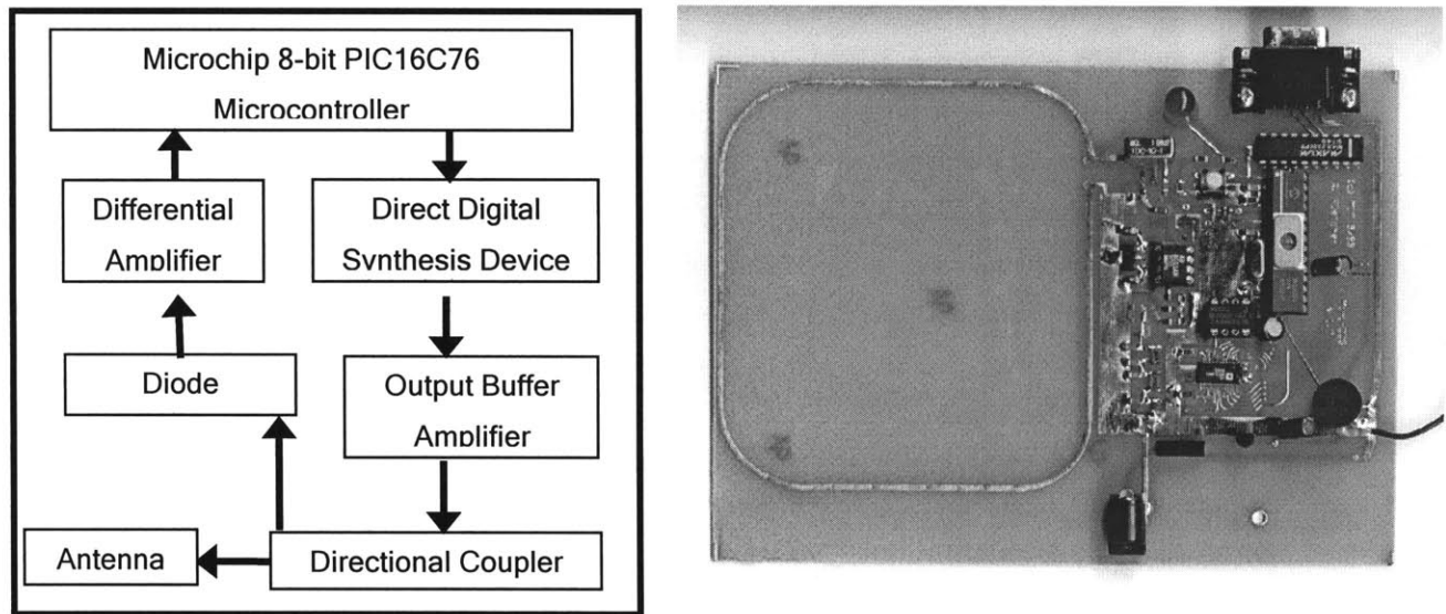
Fig. 121 Block Diagram and photo of the Mini-DDS reader
