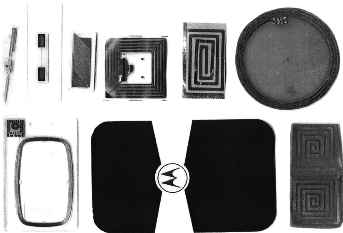
Figure 118. Photograph of a variety of electromagnetic tags, photographed to scale, including both EAS and RFID labels.
