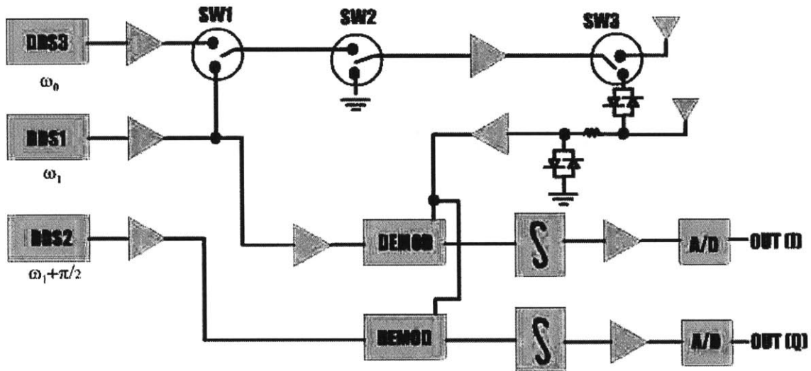
Fig. 119 Block Diagram and photograph of the wide-band harmonic and resonant tag reader, nicknamed "Sweeper."
