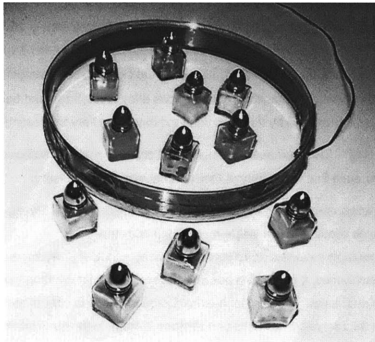
Figure 63. Portions of an October 1997 demonstration employing one dozen distinguishable items tagged with magnetoelastic resonators.
