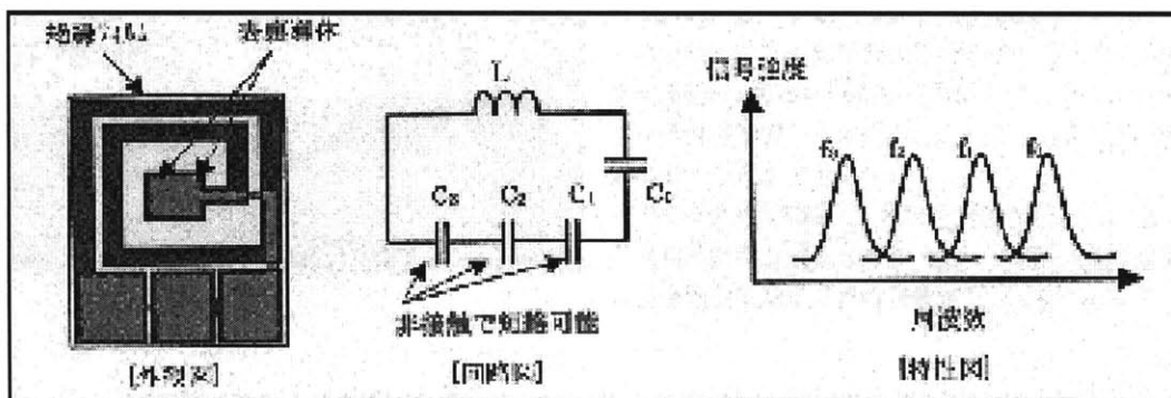
Figure 81. Sample figures from a 2002 Navitas brochure, showing their multiple capacitor tag design.
