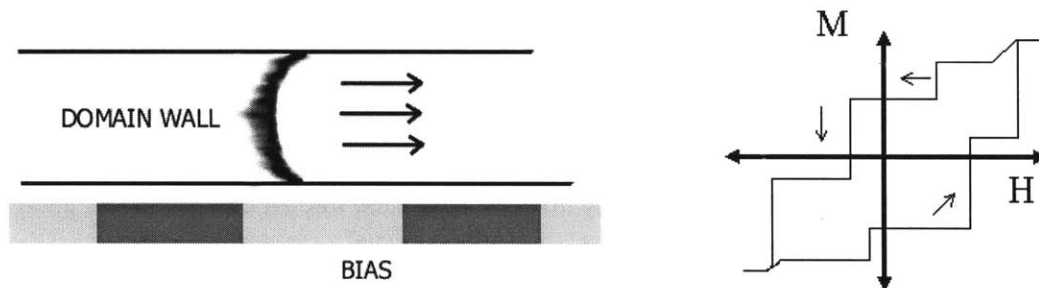
Figure 53. Schematic illustrating domain wall motion in the presence of a non-uniform magnetic field bias (left); idealized M vs H loop for this structure (right).
