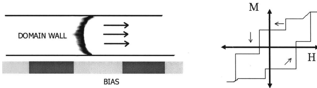
Figure 57. Schematic illustrating the basic operational concept (left); idealized M vs H loop for this structure (right).
