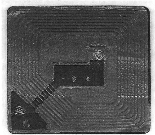
Figure 68. Photograph of planar LC tag showing lumped capacitance in center and outer corner.
