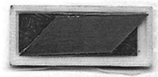
Figure 16. Electronic Article Surveillance label (Ultramax™ label by Sensormatic, Inc.) containing magnetoelastic strip and trapezoidal bias magnet.
