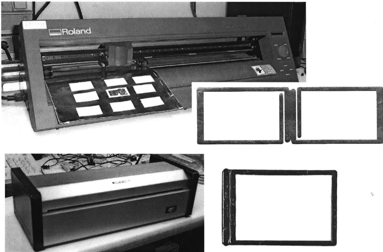
Figure 86. Equipment used to fabricate tags. (top) Roland programmable knife vinyl cutter machine and image of unfolded copper layer. (bottom) Lamination machine and image of completed tag after folding, dielectric insertion and lamination.
