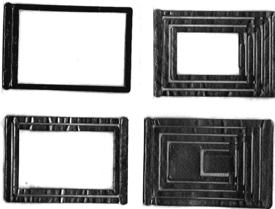
Figure 85. Example of design evolution, from a simple single-resonance structure (upper left) to a 5-resonance structure (lower right).
