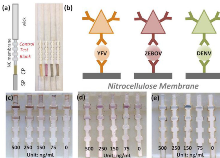
Fig. 2. Individual testing of YFV, ZEBOV, and DENV using AgNPs. a) L-R, lateral flow strips with conjugate pads (CP) loaded individually with orange, red, and green AgNPs conjugated to mAbs (strips 1-3); the conjugate pad in strip 4 is loaded with a mixture of the three AgNP-Ab conjugates and is therefore brown in color. The NC strip is 20 mm X 3 mm. b) Schematic of the sandwich assay. AgNPs of each color are specific to a pathogen marker protein. Orange, red, and green AgNPs were conjugated with mAbs specific to YFV NS1, ZEBOV GP, and DENV NS1, respectively. (c)-(e) Limit of detection (LOD) of YFV NS1, ZEBOV GP, and DENV NS1 using the different AgNP-Abs. The YFV NS1, ZEBOV GP, and DENV NS1 antigen is purchased from the Native Antigen company, IBT Bioservices, and ProSpec, respectively. Test and control antibodies were printed in lines spaced by 2.5 mm using 50 nL droplets at a 0.5 mm pitch (Digilab MicroSys) at 2 mg/mL onto HiFlow Plus nitrocellulose membrane (240 s/cm flow rate; Millipore). The repeated LOD results are presented as Supporting Information (Fig S1).
