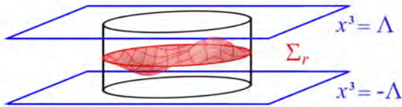
Figure 10. In their proof of the positive mass theorem, Schoen and Yau find a least area surface, \Sigma_r , with boundary, \partial\Sigma_r , lying in a cylinder of radius r , before taking r \rightarrow \infty to create a complete stable minimal surface.
