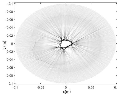
Figure 8: Sampling of the domain by the first arrival rays. The darker colors indicate more rays traveled through a particular region. Clearly the bone region has more rays passing through it than any other region of the domain. This sampling pattern is most likely causing the artifacts in the L_1 and L_2 regularized inversions.
