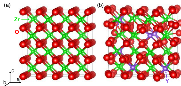
Figure 2 Atomic structures of (a) cubic \text{ZrO}_2 and (b) cubic YSZ. Zr in green, Y in purple and O in red.
