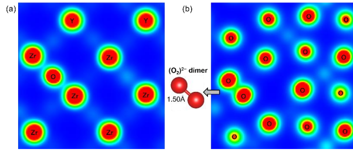
Figure 7 2D slice of charge density distributions for (100) planes (a) with an intervening O across the cation layer and (b) an O-O dimer across the oxygen layer in a Zr_{26}Y_6O_{63} supercell.
