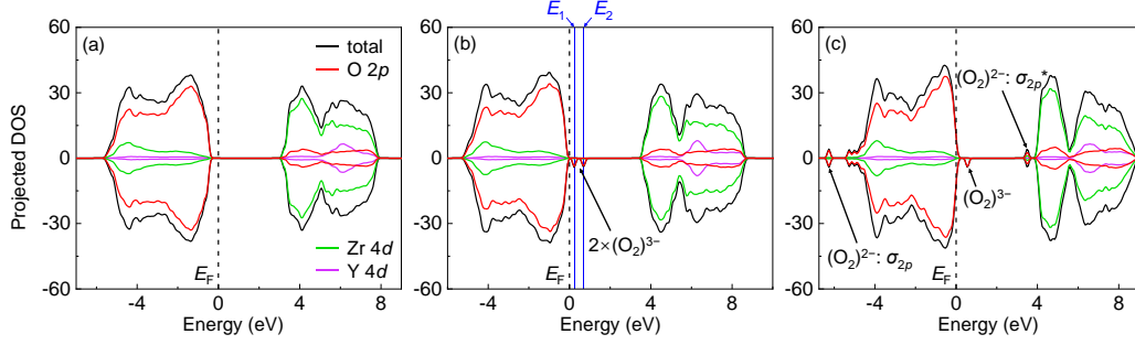
Figure 3 Calculated total DOS, and projected DOS for O 2p , Zr 4d , and Y 4d orbitals for (a) a Zr_{26}Y_6O_{61} supercell, (b) a Zr_{26}Y_6O_{62} supercell, and (c) a Zr_{26}Y_6O_{63} supercell. For y -axis, positive values denote spin-up states and negative values denote spin-down states. For x -axis, E_F is set as 0 eV.
