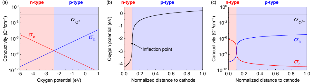
Figure 1 (a) Conductivity data of 8YSZ at 800°C. Spatial distributions of (b) \mu_{O_2} , (c) \sigma_{O_2^-} , \sigma_e , and \sigma_h inside a 10 \mu\text{m} YSZ electrolyte operated in SOEC mode under -1 \text{ A/cm}^2 at 800°C, with \mu'_{O_2} = -4.26 \text{ eV} at cathode/electrolyte interface and \mu''_{O_2} = 0.21 \text{ eV} at anode/electrolyte interface. Shaded regions in red and blue denote the n- and p-type characteristics of the minor electronic conductivity, respectively.
