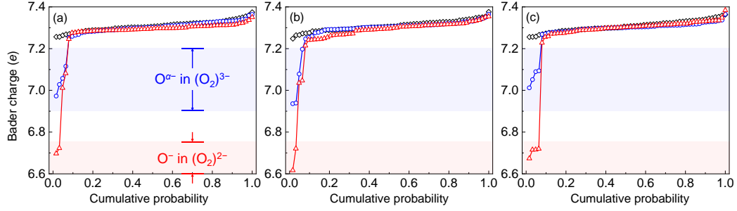
Figure 8 (a-c) Three sets of Bader charge distributions for O in Zr 26 Y 6 O 61 (black diamond), Zr 26 Y 6 O 62 (blue cycle), and Zr 26 Y 6 O 63 (red triangle). Shaded regions in blue and in red are schematic energy ranges for O α- and (O 2 ) 2- , respectively.
