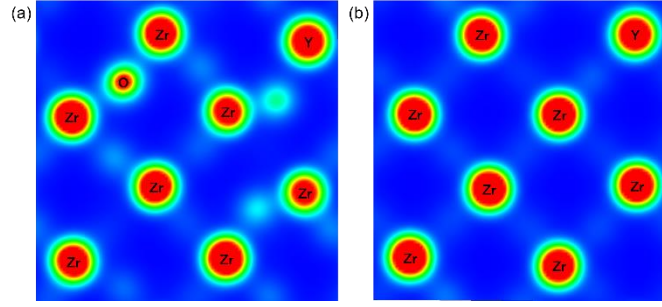
Figure 5 2D slice of charge density distributions for (100) planes across the cation layer (a) with and (b) without an intervening “special” O in a Zr_{26}Y_6O_{62} supercell.
