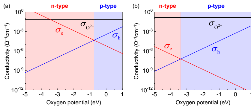
Figure 9 Conductivity data of (a) GDC and (b) LSGM at 800°C. Shaded regions in red and blue denote the n- and p-type characteristics of the minor electronic conductivity, respectively.
