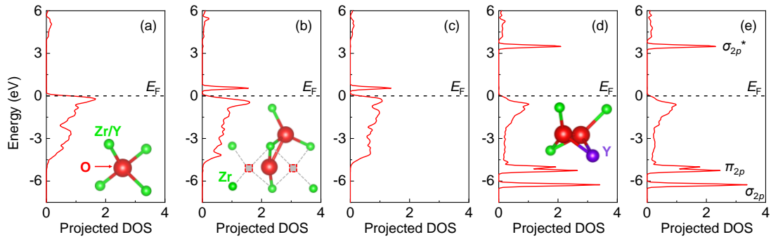
Figure 6 Projected DOS of (a) \text{O}^{2-} , (b-c) two O in (\text{O}_2)^{3-} complex, and (d-e) two O in (\text{O}_2)^{2-} in a \text{Zr}_{26}\text{Y}_6\text{O}_{63} supercell. Inset of (a): local structure of \text{O}^{2-} . Inset of (b): local structures of (\text{O}_2)^{3-} complex whose projected DOS is shown in (b-c). Inset of (d): local structures of (\text{O}_2)^{2-} whose projected DOS is shown in (d-e).
