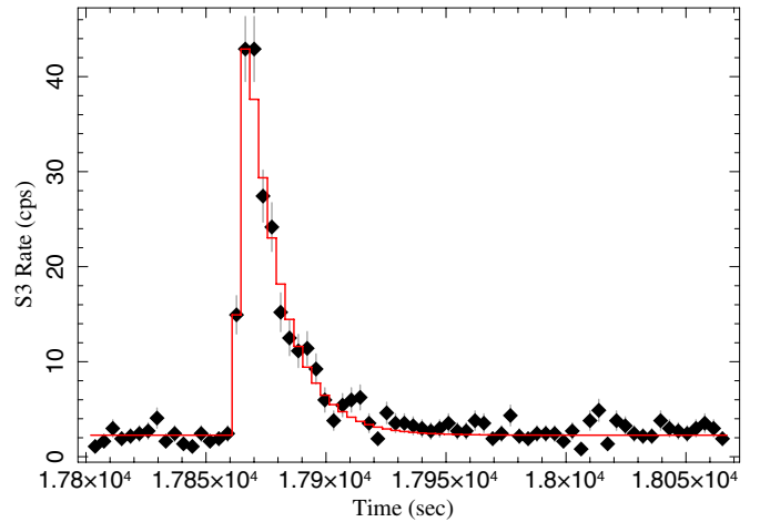
Figure 3. Zoom on the type-I X-ray burst observed in our Chandra observation of IGR J17511–3057 (2–8 keV). The time is relative to the first photon arrival time of the observation.
