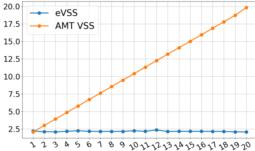
Figure 10-3: This graph plots the VSS verification round time for both eVSS and AMT VSS. The y axis is the verification round time in milliseconds and the x axis is \log_2 t . We can see AMT VSS’s verification time is slower than eVSS (i.e., \Theta(\log t) vs \Theta(1) pairings). This is the price we pay for precomputing AMT proofs much faster.
