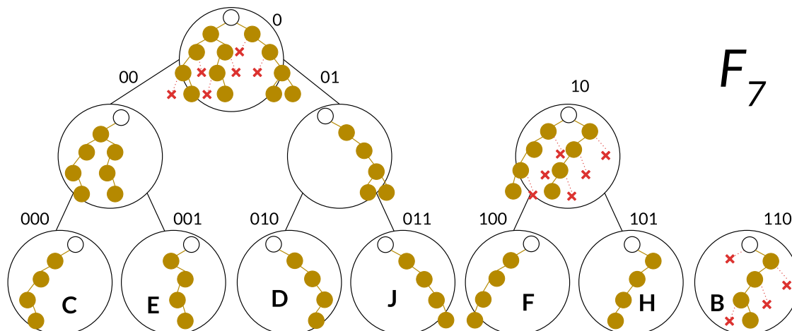
Figure 5-5: A dynamic AAS with \lambda = 2 for set \{B, C, D, E, F, H, J\} . Our AAS is a forest of PCTs with corresponding FCTs. Each node stores a prefix accumulator (and subset witness), depicted as a trie, in yellow. Root nodes store an FCT, depicted as the missing red nodes.
