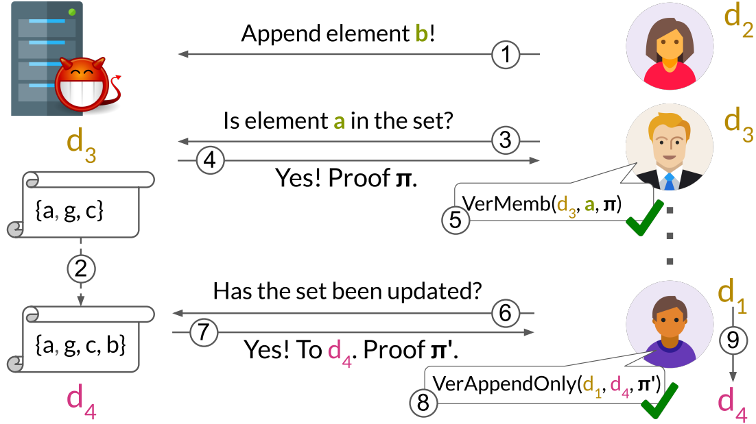
Figure 5-1: Our model: a single malicious server manages a set and many clients query the set. Clients will not necessarily have the digest of the latest set. The clients can (1) append a new element to the set, (2) query for an element and (3) ask for an updated digest of the set.
