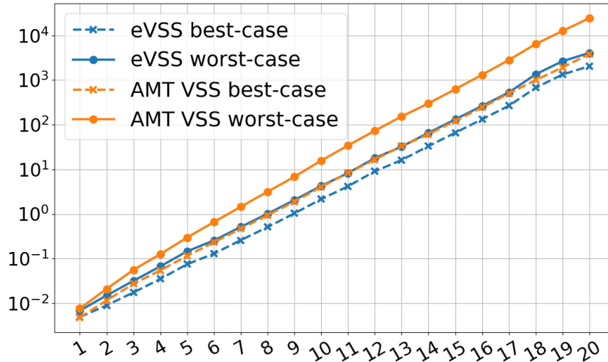
Figure 10-4: This graph shows that AMT VSS’s reconstruction time is slower than in eVSS. The y axis is the time in seconds and the x axis is \log_2 t . An interesting observation is that AMT VSS’s best-case reconstruction time is very close to eVSS’s worst-case reconstruction time (we explain in Section 10.4.2.3 why).
