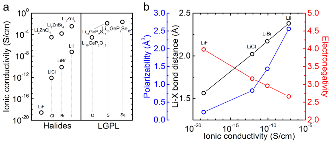
Figure 11. a) Ionic conductivity for structures with varying anions/ligands (crystalline lithium halides ( T = 400 K), 182 olivine \text{Li}_2\text{ZnM}_4 ( M = \text{Cl} , 183 \text{Br} 184 and \text{I} 185 ) ( T = 523 K) and lithium superionic conductors \text{Li}_{10}\text{GeP}_2\text{L}_{12} ( L = \text{O} , \text{S} and \text{Se} ) at room temperature 115 ). b) Halogen-atom polarizability ( \text{\AA}^3 ), 186 Li-halide bond distance ( \text{\AA} ), 186 and halogen electronegativity (Pauling scale) 187 as a function of lithium-ion
