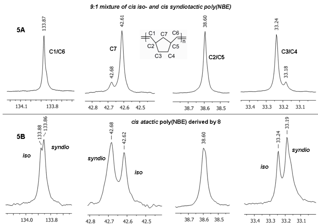
Figure 5. 5A: ^{13}\text{C} NMR spectrum ( \text{CDCl}_3 , 22 ^\circ\text{C} , 100.61 MHz) of a mixture of cis, isotactic -poly(NBE) made from 7 (90 wt%) and cis, syndiotactic -poly(NBE) made from 2 (10 wt%); 5B:
