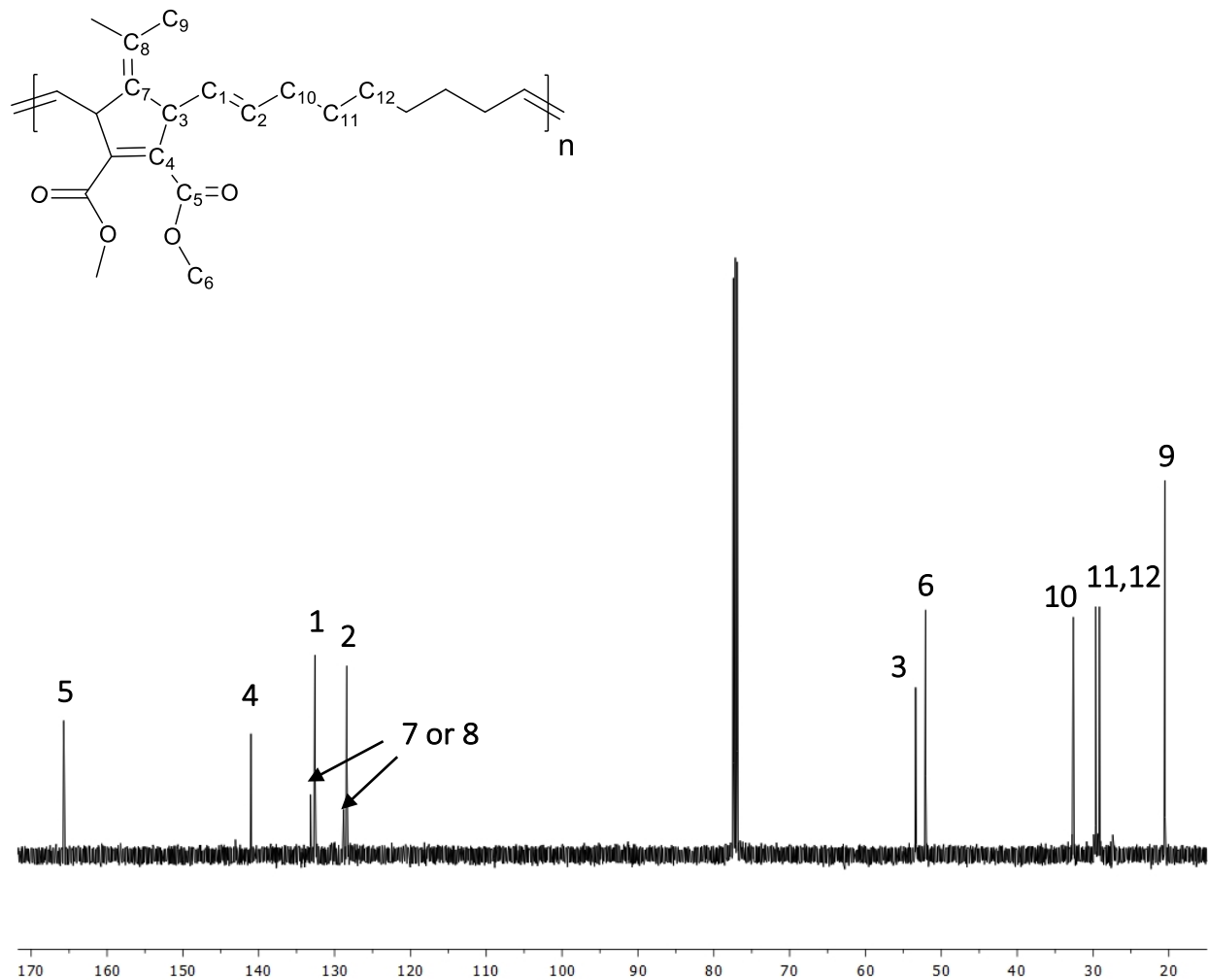
Figure S2. ^{13}\text{C} NMR spectrum of trans -poly[A- alt -B] (in \text{CDCl}_3 , 125 MHz).
