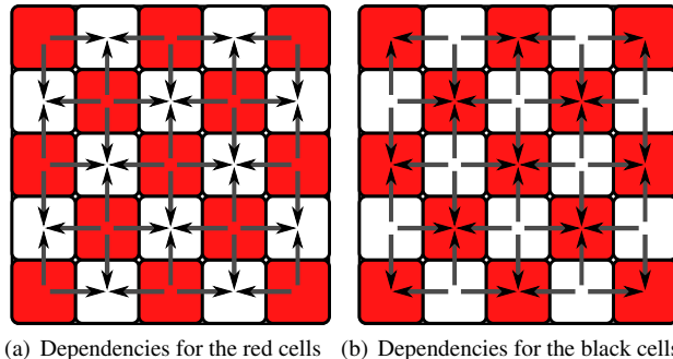
Figure 5. Checkerboard dependency pattern for Red-Black SOR. Black cells are shown in white for clarity.
