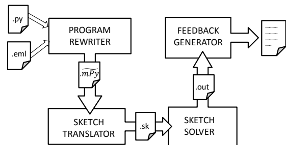
Figure 3. The architecture of our feedback generation tool.
