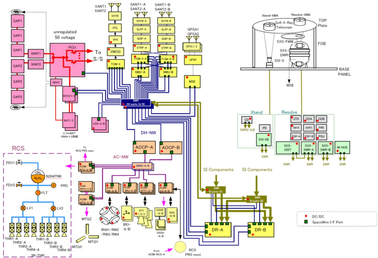
Figure 3. Function block diagram of XRISM
