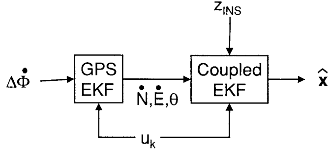
Figure 2-5: Cascaded filters indicated measurements and control inputs to each
