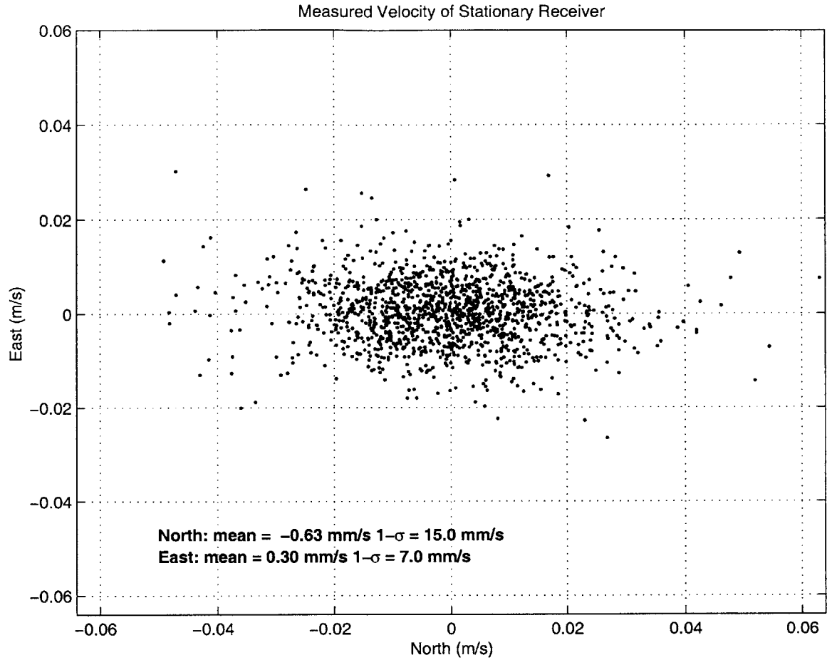
Figure 4-3: DGPS Velocity Measurements of a Stationary Antenna
