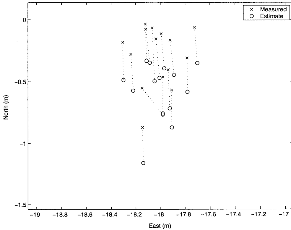
Figure 4-15: Final position of control experiments: \circ indicates estimated value, \times is the measured value for validation
