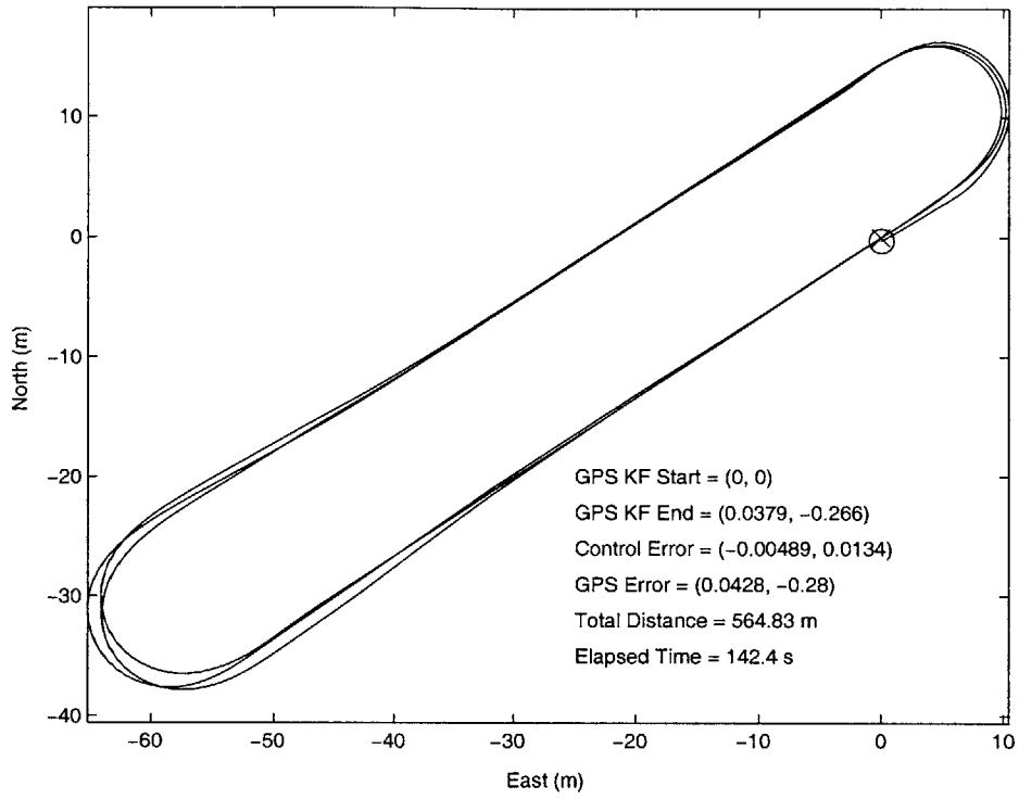
Figure 4-5: Integrated GPS velocity from differential Doppler measurements
