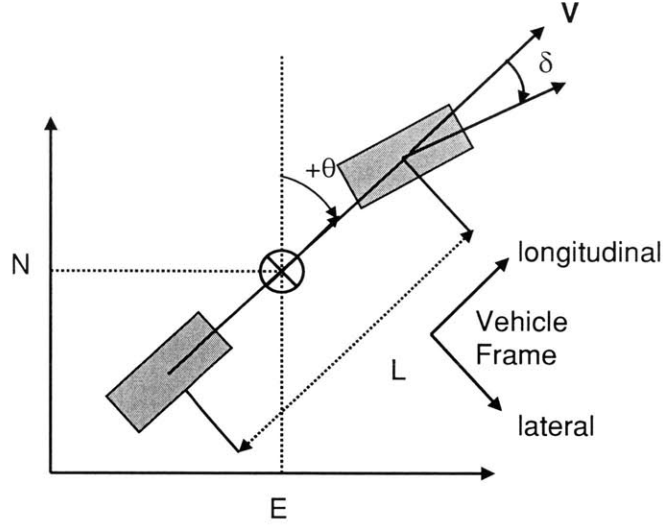
Figure 2-4: Rigid body motion of Ellis bicycle model with identified parameters
