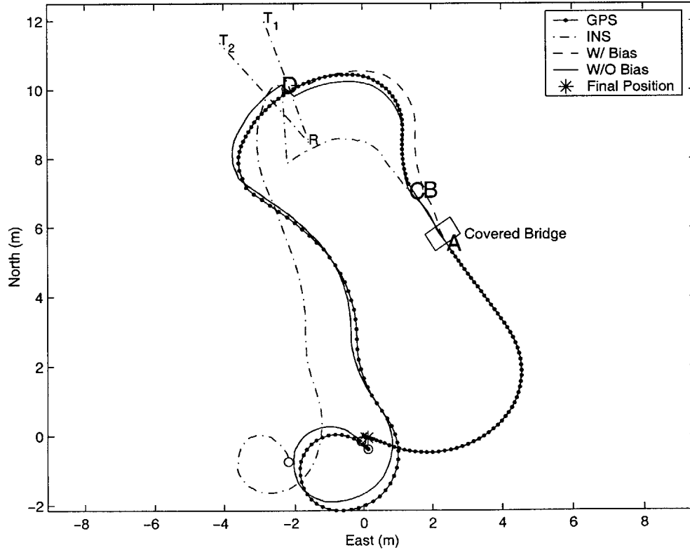
Figure 4-12: Position results of GPS and Coupled EKF - Run 37
