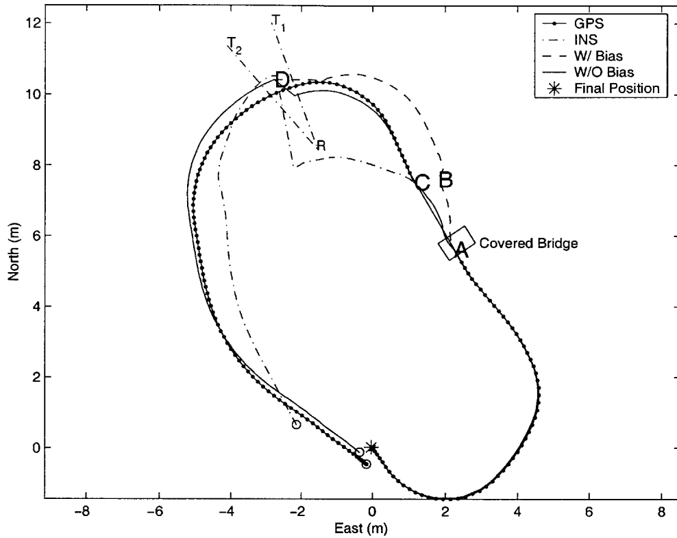
Figure 4-13: Position results of GPS and Coupled EKF - Run 39
