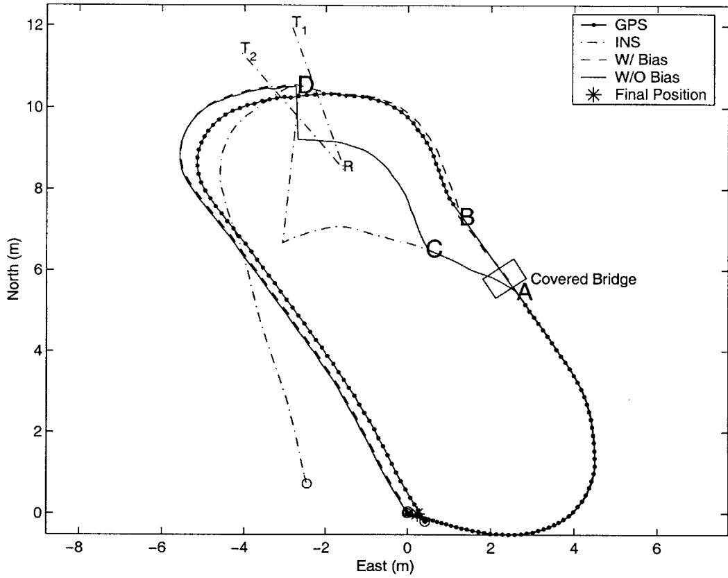
Figure 4-7: Position results of GPS and Coupled EKF - Run 33
