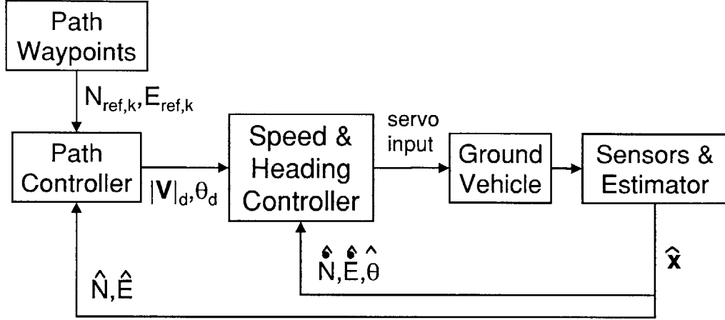
Figure 3-4: Ground vehicle closed-loop position control
