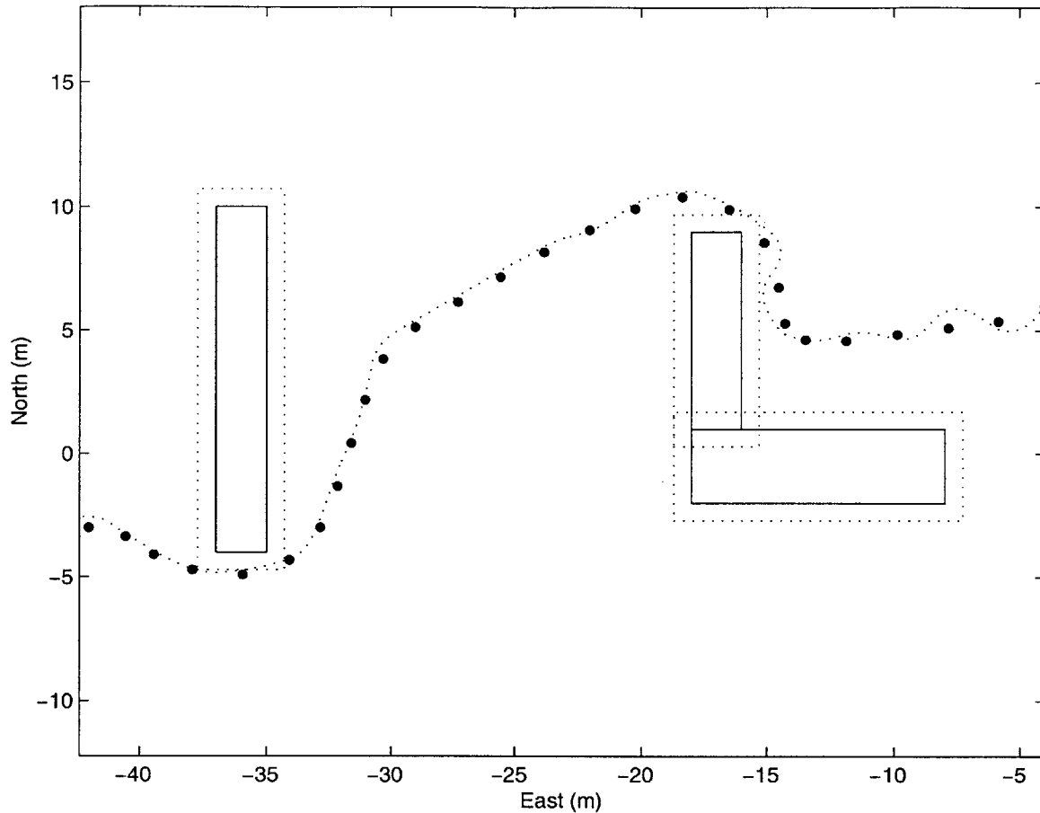
Figure 4-19: Test of dynamic planning algorithm that adjusts plan while maneuvering
