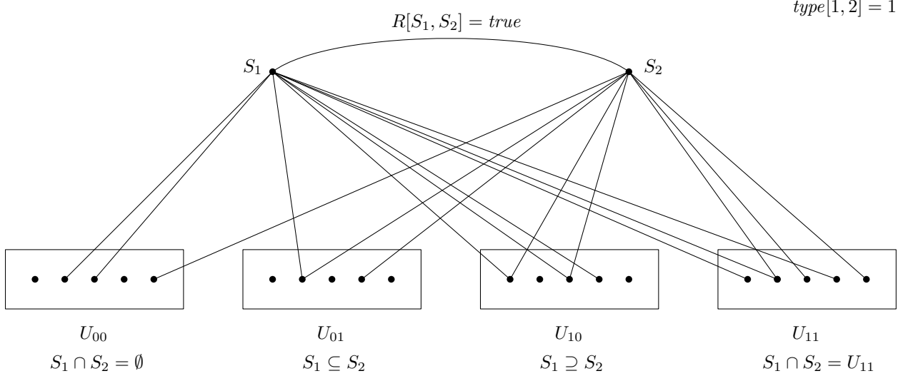
Figure 4: An example of a solution to a Hybrid Problem instance, when k = 2 . In sub-universes U_{00}, U_{01}, U_{10}, U_{11} , sets S_1 and S_2 are solutions of BP[00] (Set Disjointness), BP[01] (Set Containment), BP[10] (Set Containment in the reversed direction) and BP[11] (2-Set Cover), respectively. And type[1, 2] = 1 specifies that the predicate R on (S_1, S_2) must be true.
