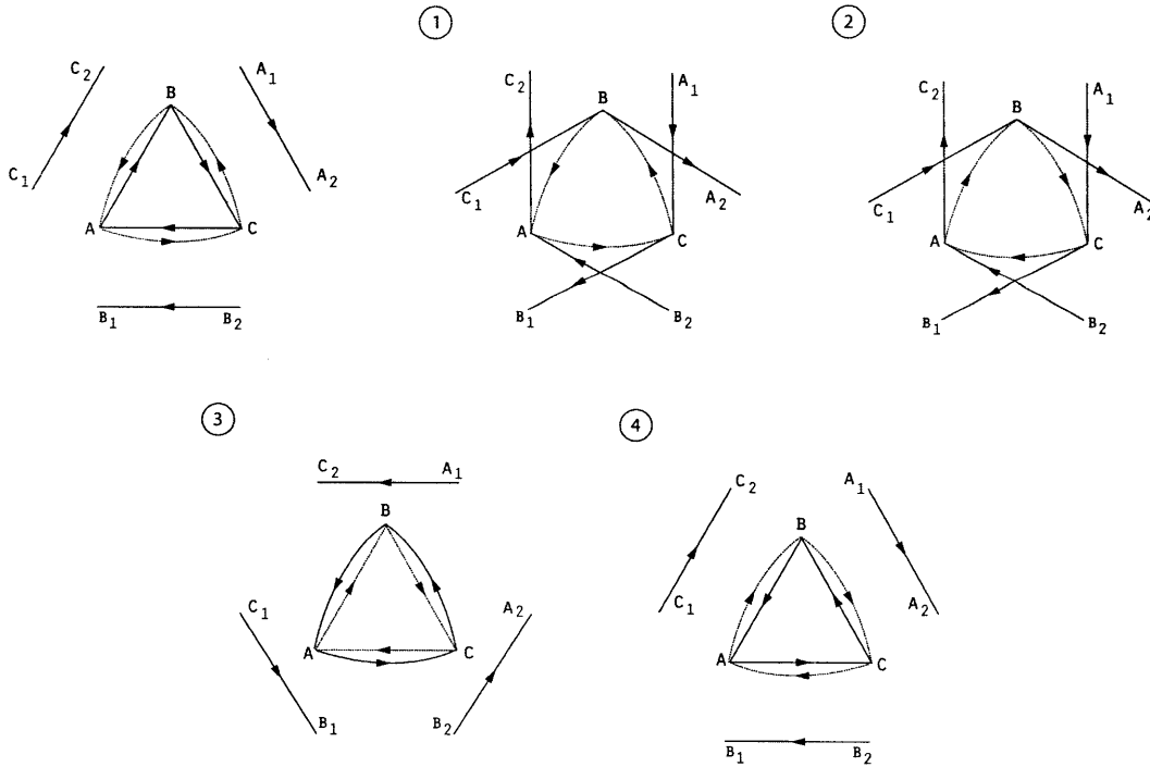
Figure 7-1: The sequence of operations that flips a strong triangle. Dotted lines indicate negative edges, while solid lines indicate positive edges.
