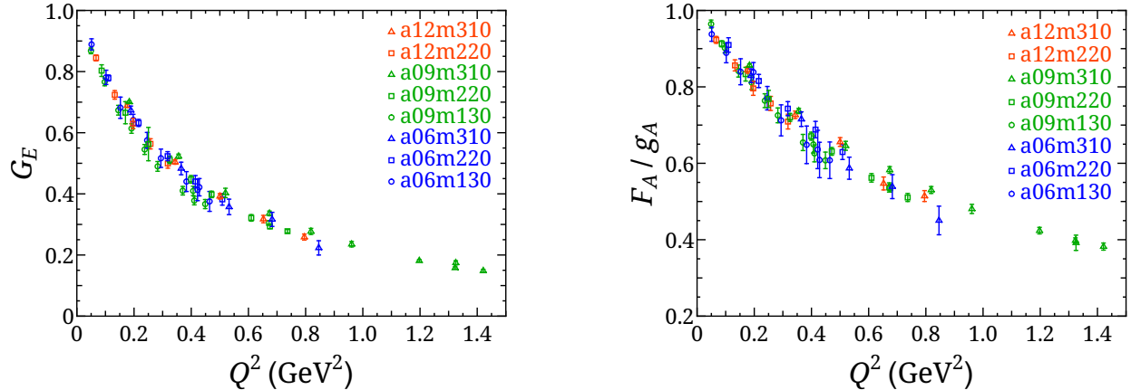
FIG. 4. Electric (left) and isovector axial (right) form factors of the nucleon vs Q^2 = -q^2 . Data from Ref. [66, 75].
