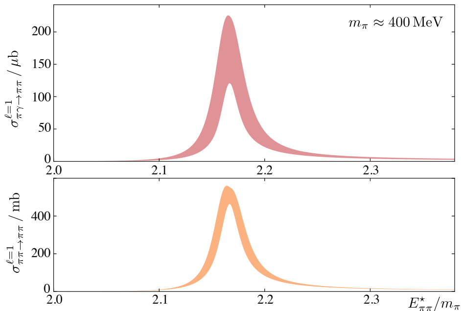
FIG. 6. The upper and lower panels show the \gamma^*\pi^+ \rightarrow \pi^+\pi^0 and l = 1 elastic \pi\pi scattering cross sections, respectively, as a function of \pi\pi energy, with the \rho resonance clearly visible [142].
