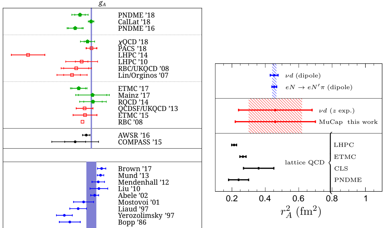
FIG. 5. Status of lattice-QCD calculations of g_A (left) and r_A^2 (right), together with non-lattice determinations. Left: Filled green (unfilled red) lattice-QCD results have (in)complete error budgets. The violet line in the upper panel is the PDG average of the results in the bottom panel, in which the scale is blown up by a factor of 10. Right: As discussed in the text, the error bars on r_A^2 from dipole fits are underestimated and the two small lattice-QCD error bars stem from incomplete error analyses (critiqued below). The references for r_A^2 from top to bottom are as follows: “ \nu d and eN \rightarrow eN'\pi (dipole)” [50], “ \nu d ( z exp.)” [58], “MuCap this work” [59], LHPC [62] (NB: one lattice spacing and M_\pi = 317 MeV), ETMC [63] (NB: no strange sea and a small volume such that M_\pi L < 3 ), CLS [64], PNDME[65]. From Refs. [77] (left) and [59] (right, adapted with permission).
