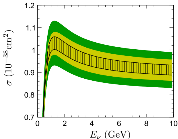
FIG. 3. Quasielastic neutrino-neutron cross section assuming current uncertainties for all crucial inputs except r_A^2 , for which a 20% uncertainty is assumed. The hatched (yellow) error band stems from this putative r_A^2 (all other inputs); the green band is the sum in quadrature. From Ref. [59].
