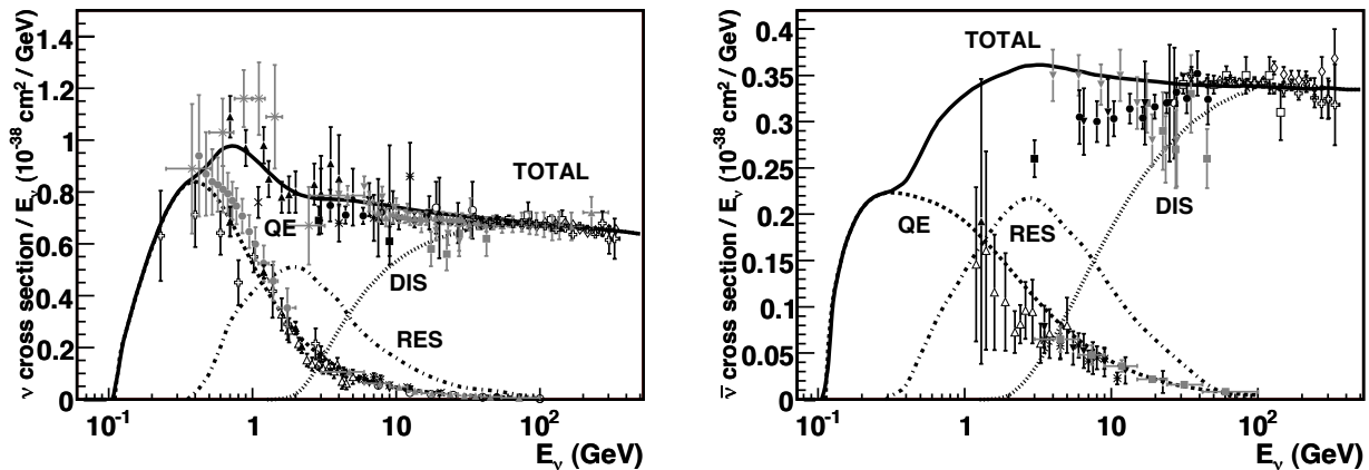
FIG. 2. Cross sections vs neutrino energy (left) or antineutrino energy (right), showing the relative contributions of the underlying processes quasielastic scattering, resonance production, and deep-inelastic scattering [35].
