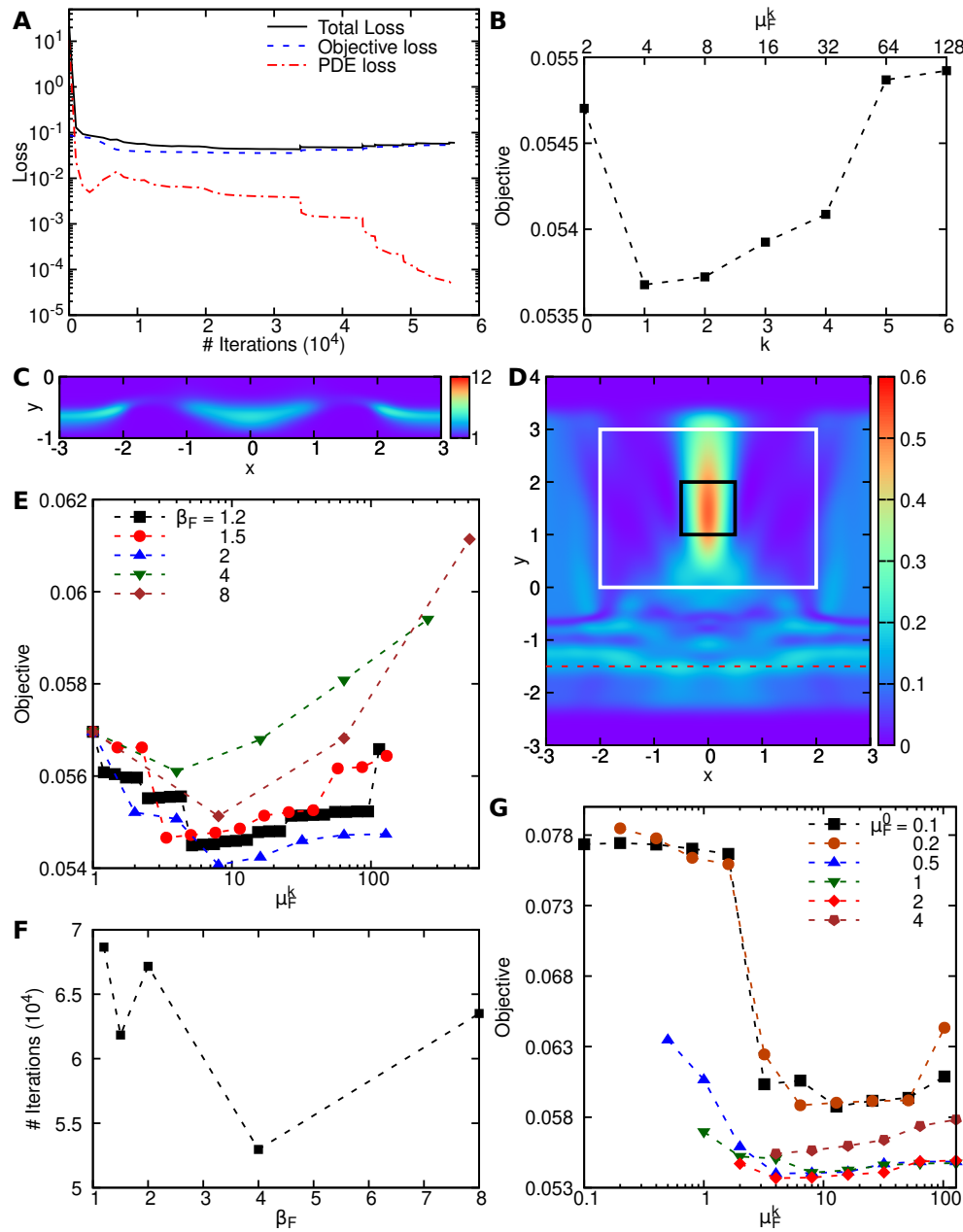
FIG. 5. hPINN for the inverse design of holography via the penalty method. (A) to (D) The results of \mu_F^0 = 2 and \beta_F = 2 . (A) The losses versus the number of optimization iterations. (B) the objective value after the network is trained with \mu_F^k , (C) the optimized permittivity function \varepsilon at k = 1 , and (D) the corresponding electric field |E|^2 . (E) The objective value versus \mu_F^k when using different values of \beta_F . (F) The total number of optimization iterations (which is proportional to the computational cost) for different \beta_F . (G) The objective value versus \mu_F^k for different values of \mu_F^0 .
