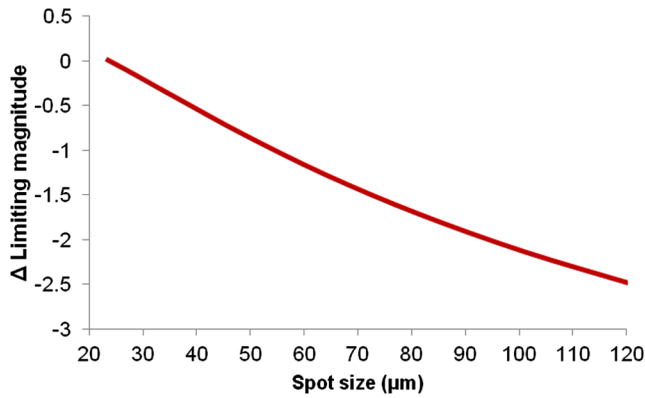
Fig. 14 The predicted impact of spot size on the system performance in terms of limiting magnitude for a constant integration time and set of atmospheric conditions. The limiting magnitude degrades substantially as the spot size grows, smearing the signal over additional pixels and decreasing the signal-to-noise ratio.
