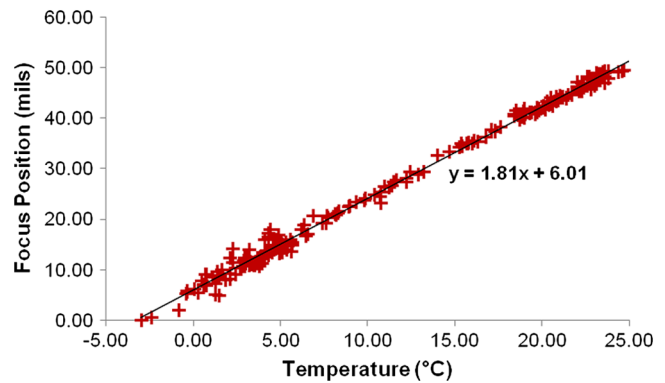
Fig. 13 Empirical relationship between mirror positions along the optical axis (Tertiary Mirror z —Secondary Mirror z ) and average temperature of the telescope structure.
