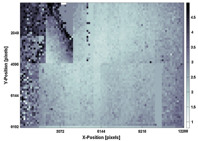
Fig. 16 Map of normalized spot size across the focal plane. The data points show the mean spot size in 128 \times 128 pixels averaged over five frames of stellar imagery. The pixel gray scale is in units of relative PSF. The two chips in the upper left corner exhibit significantly degraded spot sizes compared with the remainder of the focal plane. Current hypothesis suggests that the performance impact is caused by the chip alignment relative to the focal plane, which explains the discontinuity observed around pixel coordinate x = 2000 and 4000 . The remainder of the focal plane displays the expected radial symmetry that is consistent with optimal mirror alignment.
