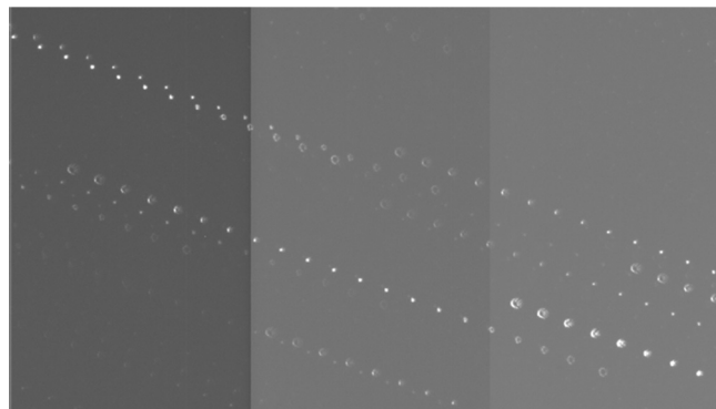
Fig. 6 Actual data showing steps through tertiary mirror y (along the optical axis) to find the minimum spot size on average across the field.
