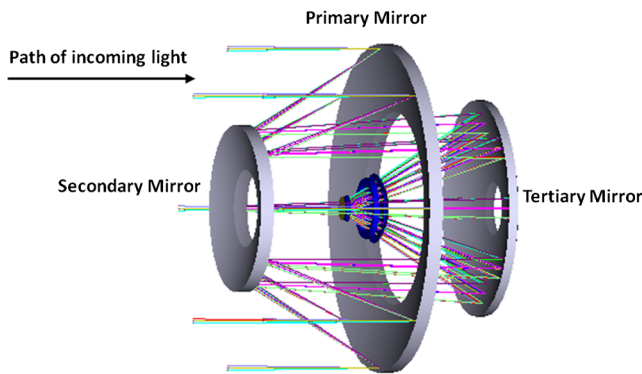
Fig. 1 Optical layout of the SST. Light enters the system from the left in this image.
