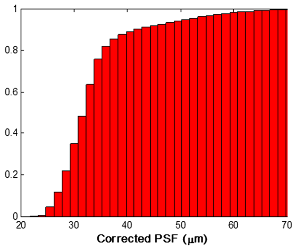
Fig. 15 Cumulative histogram of PSF size (rms diameter in units of \mu\text{m} ). The data set is comprised of the average PSF in each images observed on 2012 days 284 to 286. The median corrected PSF value after correcting for airmass is 33 \mu\text{m} , which corresponds to 0.3 magnitudes off optimal performance. The system maintains a PSF less than 42 \mu\text{m} for 90% of the time, which corresponds to 0.6 magnitudes off optimal expectations (which is set for good seeing conditions.)
