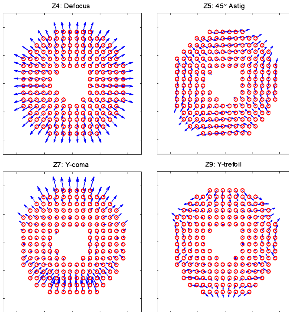
Fig. 3 The contribution to image blur of each aberration is assessed from the rms of the subaperture spot displacements at each point on the wavefront. The figure on the top left shows the effect of Z4 (defocus): a radially symmetric shift outward in the subaperture spot position. The figure on the top right shows Z5 (astigmatism at 45^\circ ). In the bottom row, the figure on the left shows Z7 ( y -coma) and the figure on the right shows Z9 ( y -trefoil). The amount of astigmatism, coma, etc. that is displayed in each figure is selected for the purpose of illustration, and do not represent the magnitude of aberrations present in an actual system.
