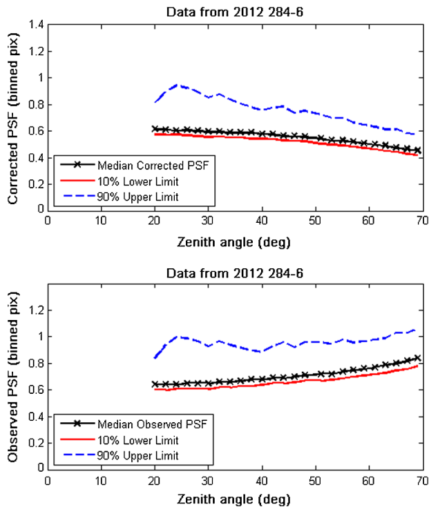
Fig. 12 The performance of the elevation correction is demonstrated in the plot of spot size as a function of zenith angle for all observations on the typical nights of 2012 days 284 to 286. The upper panel shows the PSF after applying the correction for airmass, and the lower panel shows the observed (uncorrected) values. The atmospheric correction assumes the standard model where the PSF increases proportional to (\text{airmass})^{0.6} . The slight decrease in spot size at low elevation (large zenith angle) is due to a combination of improved alignment performance at low elevation and overestimation of the atmospheric correction on a night with good seeing conditions. The PSF is reported as rms diameter in units of \mu\text{m} .
