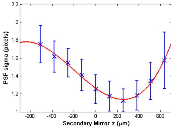
Fig. 8 In-focus PSF size measured on actual data for coordinated moves of tertiary and secondary mirrors along the optical axis. The total path length remains constant, i.e., defocus aberration is unchanged while the spot size changes due to spherical aberration.
