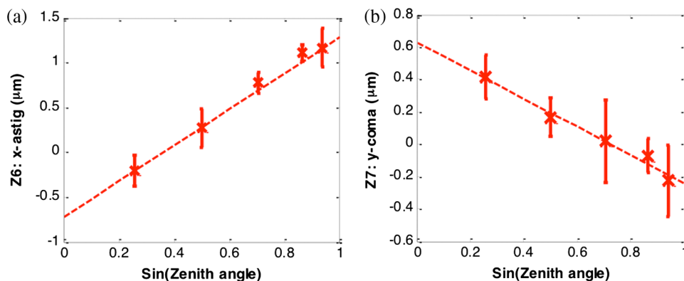
Fig. 11 (a) The measured Z6 term and (b) measured Z7 term show clear trends as a function of the zenith angle.
