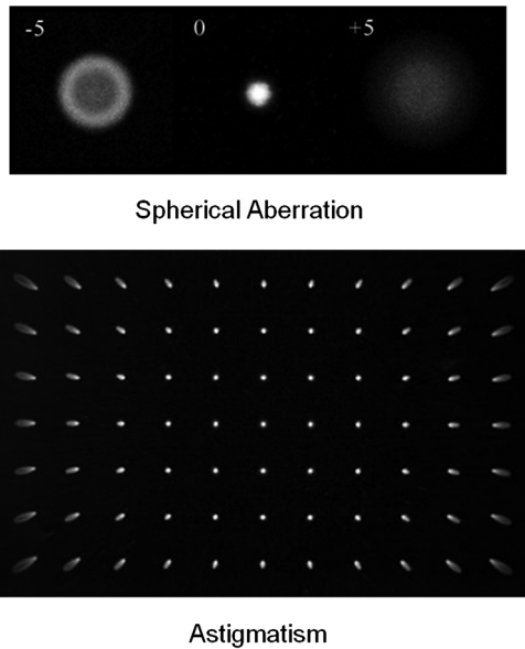
Fig. 5 The top panel shows the Zemax prediction for PSF with spherical aberration for in-focus and out-of-focus images. The bottom panel shows the Zemax prediction for misalignment induced astigmatism across the focal plane.
