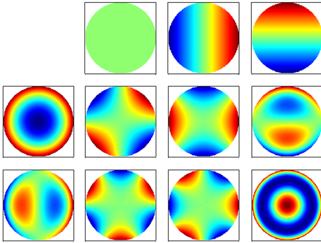
Fig. 2 Zernike polynomial representation of an aberrated wavefront. The Zernike numbering system follows the Noll convention. 12
