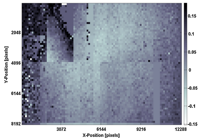
Fig. 17 Map of the impact to the magnitude limit of observations due to the spot size variation across the focal plane. The pixel gray scale is in units of relative magnitude. (White pixels indicate no data.) The magnitude limit is computed from a model of the telescope system performance, which is a function of parameters including the telescope aperture size and focal ratio, the noise characteristics of the imager, and the PSF size. The measured PSF that is observed at each location on the focal plane (Fig. 16) is provided as input to the telescope model, producing a map of the expected magnitude limit across the focal surface. The spatial variation in PSF performance that is observed in Fig. 16 results in the estimated variation in magnitude limit shown in this figure.
