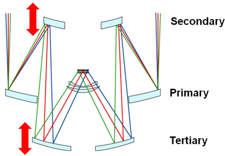
Fig. 7 The coordinated translation of secondary and tertiary mirrors along the optical axis is necessary for removing spherical aberration.
