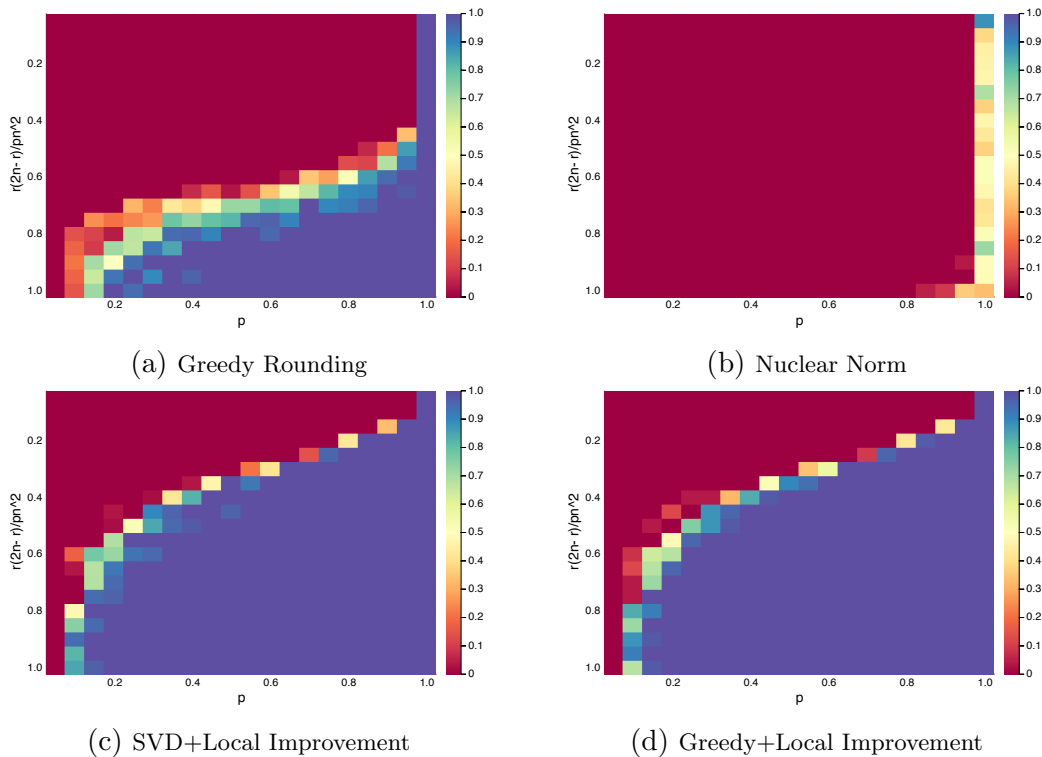
Figure 2 Prop. matrices recovered with \leq 1\% relative MSE (higher is better), for different values of p (x-axis) and r(2n-r)/pn^2 \propto 1/n (y-axis), averaged over 25 rank- r matrices.
