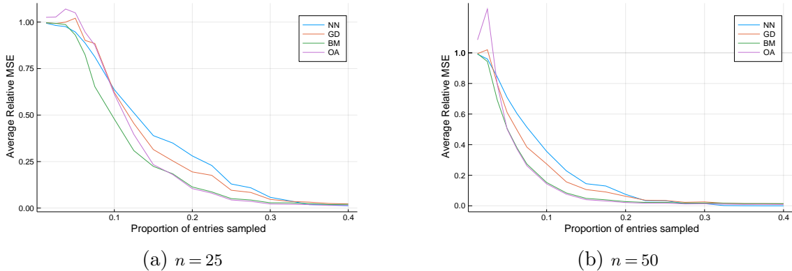
Figure 4 Average relative MSE for nuclear norm (NN), greedy rounding (GD), Burer-Monterio (BM), and outer-approximation (OA) when imputing a rank-1 n \times n matrix. All results are averaged over 25 matrices.
