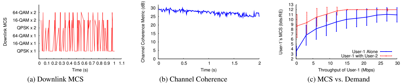
Figure 9: Insights into Rate Adaptation: (a) Trace of Downlink MCS for a user over time; (b) Channel Coherence metric of a USRP placed at the user’s location over time; (c) Mean downlink MCS (bits/resource element) across demand, with and without another high-demand user.
