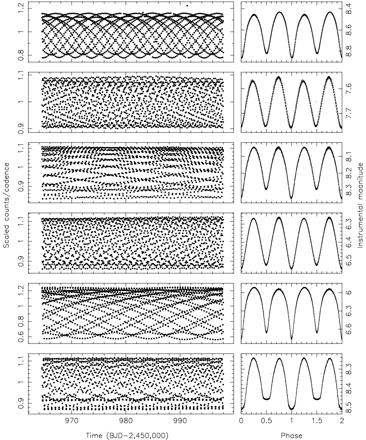
Figure 4. Similar to Figure 2 for EBs classified as overcontact (OC). The stars are, from top to bottom, KID 6106771 ( P = 0.26384 d), KID 6265720 ( P = 0.31237 d), KID 10447902 ( P = 0.33745 d), KID 3732732 ( P = 0.39617 d), KID 6671698 ( P = 0.47153 d), and KID 3127873 ( P = 0.67146 d).
