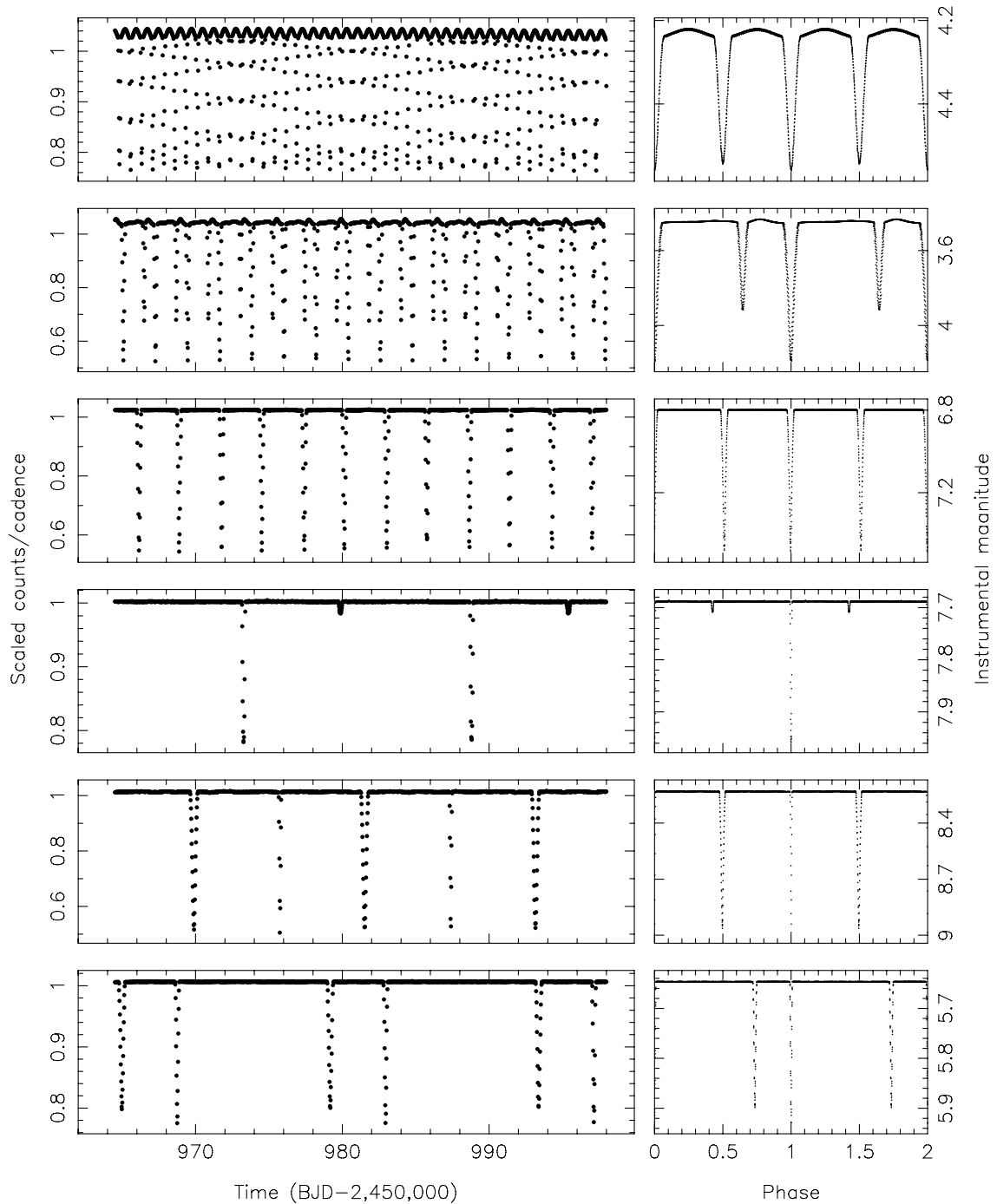
Figure 2. Example light curves showing EBs classified as detached (D). The left-hand panels show the data in normalized flux units plotted as a function of time. The right-hand panels show the phased light curves in arbitrary magnitude units as in Figure 1. Two binary cycles are shown for clarity. The stars are, from top to bottom, KID 5513861 ( P = 1.51012 d), KID 4544587 ( P = 2.19074 d), KID 4445630 ( P = 5.62746 d), KID 6841577 ( P = 15.5376 d), KID 5955321 ( P = 11.6347 d), and KID 9509207 ( P = 14.1991 d).
