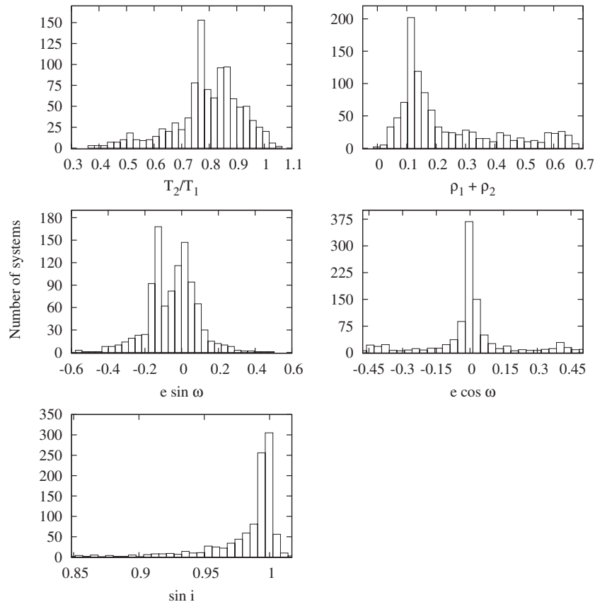
Figure 15. Distributions of the five principal parameters for detached/semi-detached binaries. See the text for discussion.
