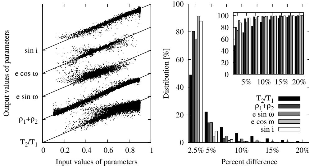
Figure 10. EBAI performance on a test set of 10,000 detached EBs distinct from the training sample. Despite the increased morphology complexity, the network still yields a statistically significant result: 90% of all systems have errors in all five parameters smaller than 10%.
