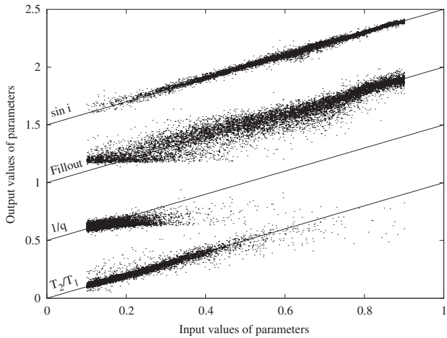
Figure 8. EBAI performance on a test set of 10,000 overcontact EBs distinct from the training sample. The correlation between input values and recognized output values is shown for each parameter and offset by 0.5 for clarity. Labeled guidelines representing ideal performance are provided for easier comparison. The observed trends and areas of increased scatter are well understood and discussed in the text.
