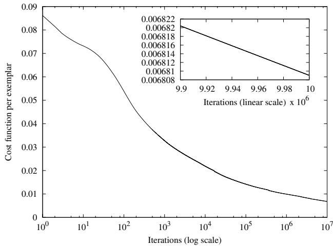
Figure 7. Neural network learning curve for overcontact binaries. The cost function is defined as the average deviation per parameter per exemplar. The data on the main plot are depicted in log scale, while the data in the inset are in linear scale. The network was trained on 10,000 exemplars for 10,000,000 iterations.
