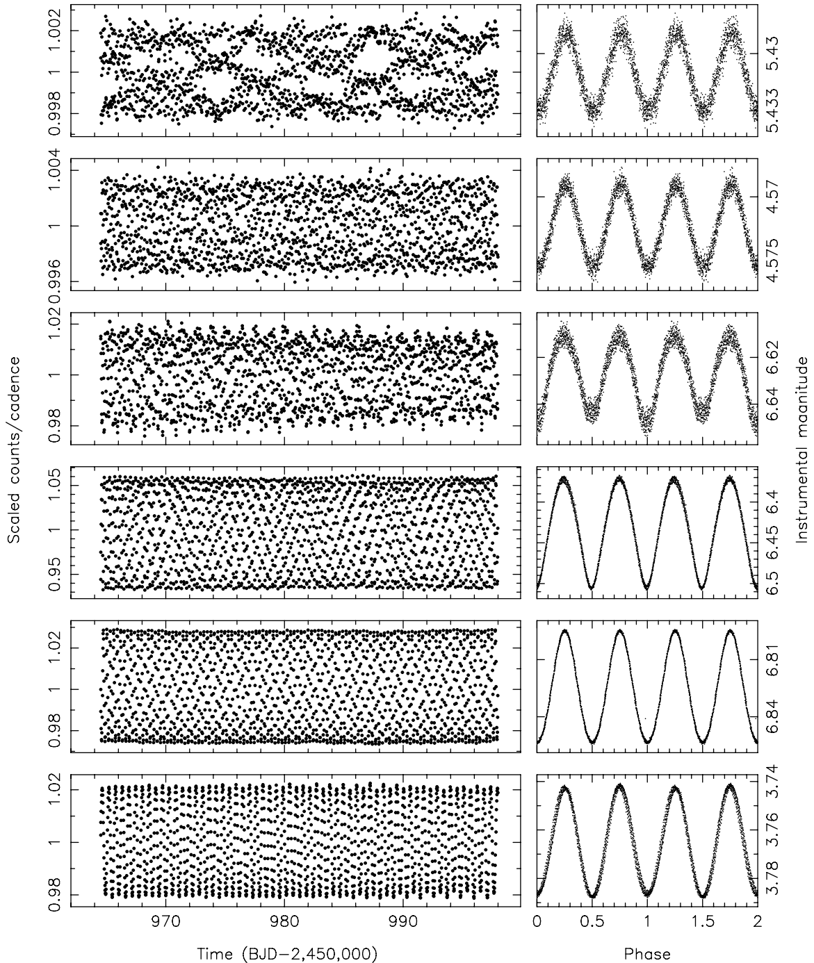
Figure 5. Similar to Figure 2 for EBs classified as ellipsoidal (ELV). The stars are, from top to bottom, KID 9508052 ( P = 0.27999 d), KID 4661397 ( P = 0.292301 d), KID 4940217 ( P = 0.37873 d), KID 9071104 ( P = 0.385229 d), KID 10389982 ( P = 0.443392 d), and KID 4273411 ( P = 1.21973 d).
