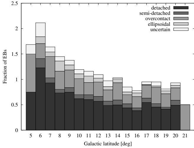
Figure 12. Distribution of EBs as function of galactic latitude, normalized to the number stars per degree observed by Kepler . Morphology types are denoted with different gray scales. The trend is a consequence of the Kepler target selection.
