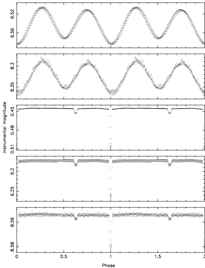
Figure 1. Examples of spurious detections of contaminating EBs. The y-axis is an arbitrary instrumental magnitude scale given by y = -2.5 \log(\text{counts}) + 26.0 . The top two stars and their ephemerides are KID 7546791 ( T_0 = 54964.6060 , P = 0.24231 ) and KID 7546789 ( T_0 = 54964.6023 , P = 0.24233 ), respectively. KID 7546791 is most likely the true binary since it is about 1.75 mag brighter than KID 7546789. The bottom three stars are KID 9851142 ( T_0 = 54968.8631 , P = 8.48517 ), KID 9851126 ( T_0 = 54968.8573 , P = 8.48516 ), and KID 9851123 ( T_0 = 54968.8558 , P = 8.48027 ), respectively. The likely true binary in this case is KID 9851142. There were 61 occurrences in the sample that were detected and removed.
