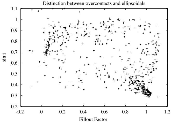
Figure 14. Correlation between the fillout factor F and \sin i . The area at bottom right corresponds to ellipsoidal variables.
