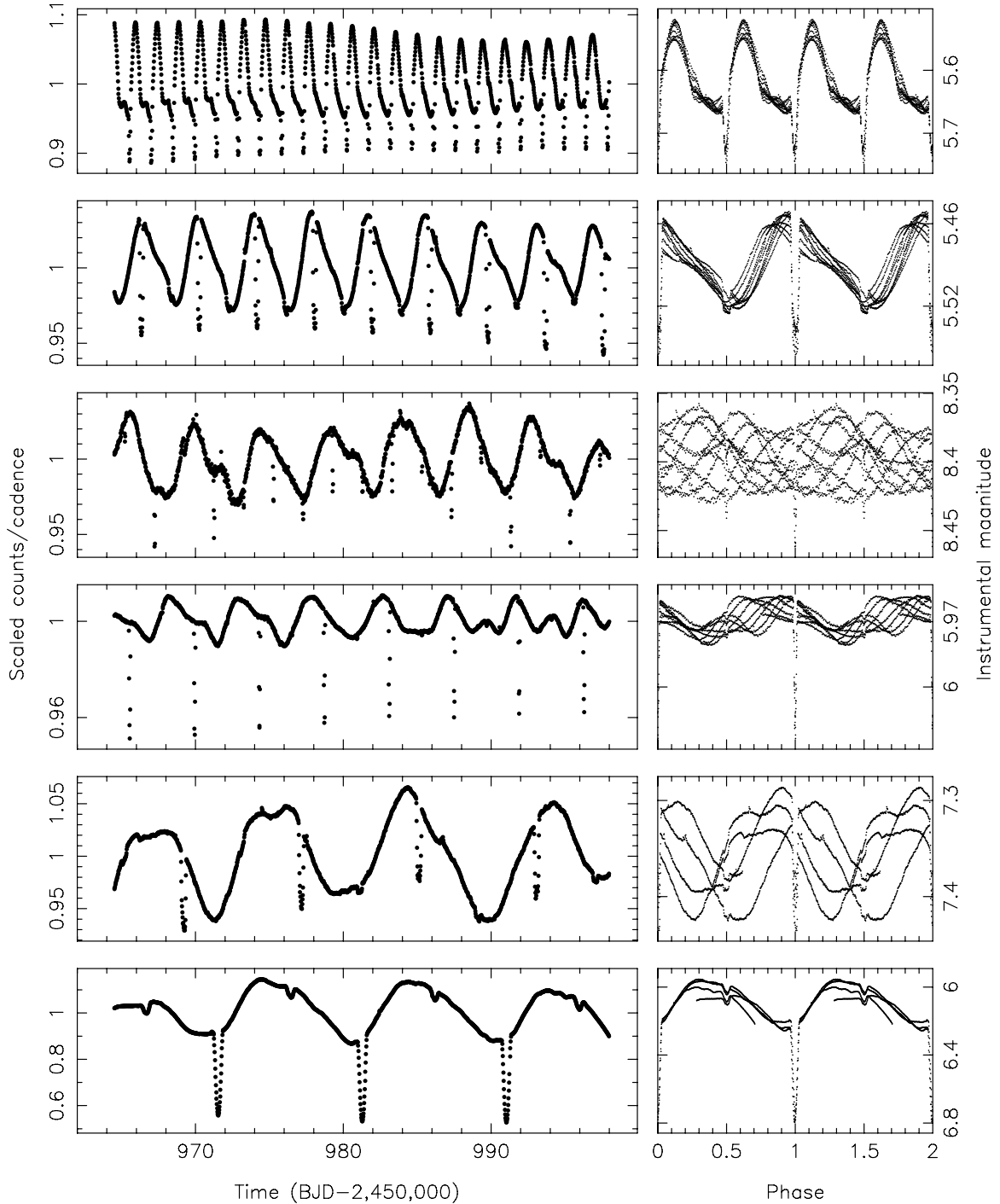
Figure 6. Similar to Figure 2 for intrinsically variable EBs. The stars are, from top to bottom, KID 9137992 ( P = 2.94213 d), KID 7940533 ( P = 3.90567 d), KID 3427776 ( P = 4.01626 d), KID 5768927 ( P = 4.39063 d), KID 9576197 ( P = 7.96253 d), and KID 6197038 ( P = 9.77901 d).
