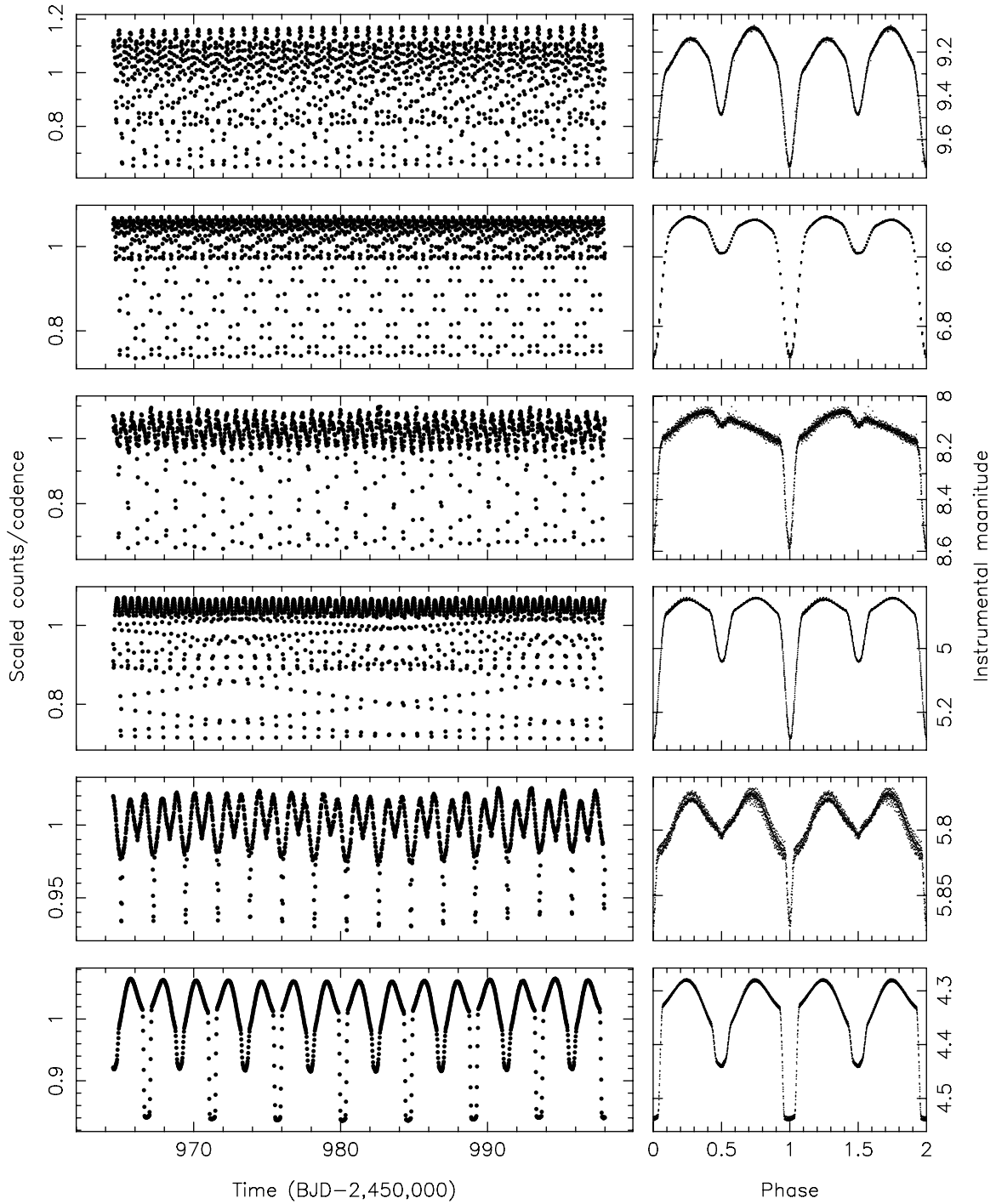
Figure 3. Similar to Figure 2 for EBs classified as semi-detached (SD). The stars are, from top to bottom, KID 3218683 ( P = 0.77167 d), KID 8074045 ( P = 0.53638 d), KID 9328852 ( P = 0.64581 d), KID 4729553 ( P = 0.96131 d), KID 11175495 ( P = 2.19126 d), and KID 8868650 ( P = 4.44741 d).
