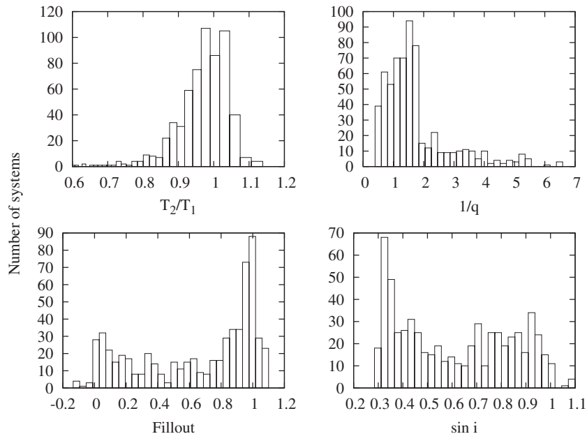
Figure 13. Distributions of the four principal parameters for overcontact binaries and ellipsoidal variables. See the text for discussion.
