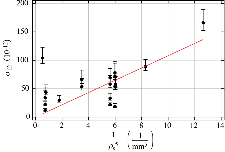
Figure 5-17: Observed frequency noise \sigma_{f2} as a function of 1/\rho_s^5 . The data exhibit the expected linear scaling at small separation (right hand side of the plot). At large separation, \sigma_{f2} levels off because relativity, and B_2 start to dominate. The straight line shown is a fit to the data constrained to go through the origin.
