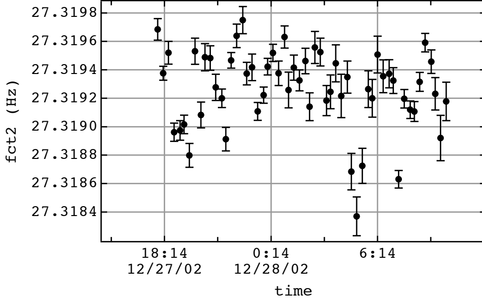
Figure 6-1: Typical sequence of measured cyclotron frequency difference vs time. The standard deviation of the points is 7 \times 10^{-11} and the total data set determines the difference frequency with a relative precision of 1 \times 10^{-11} .
