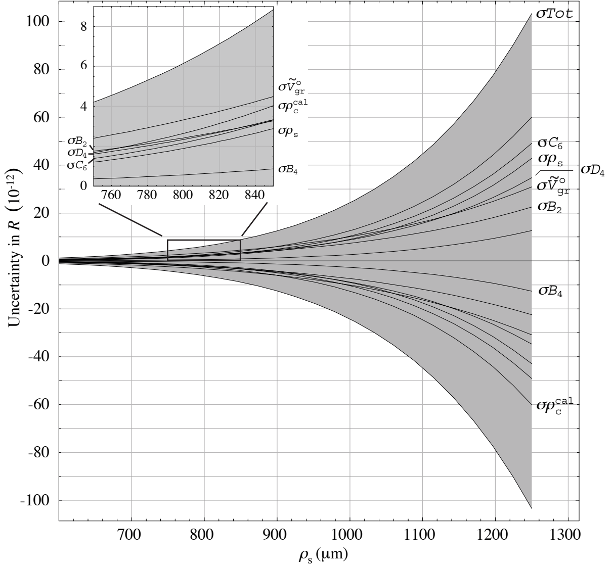
Figure 5-7: Uncertainty band on \Delta\omega_{\text{ct}2}/\omega_{\text{ct}2} vs \rho_s from trap imperfections. Individual contributions from \sigma D_4 , \sigma \tilde{V}_{\text{gr}}^o , \sigma C_6 , \sigma B_2 , \sigma B_4 , \sigma \rho_s and \sigma \rho_c^{\text{cal}} are plotted and the gray band is the total uncertainty. The plot is symmetric upon reflection about the x-axis and the label positions indicate the sign of each contributions. For instance, if \rho_c^{\text{cal}} increased, the measured ratio would be smaller.
