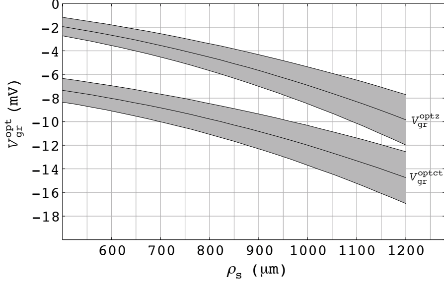
Figure 5-6: V_{\text{gr}}^{\text{optct}} and V_{\text{gr}}^{\text{optz}} as a function of \rho_s . The plotted band are the 1\sigma uncertainties on these voltages with contributions from \sigma D_4 , \sigma \tilde{V}_{\text{gr}}^{\circ} , \sigma C_6 , \sigma B_2 , \sigma B_4 , \sigma \rho_s and \sigma \rho_c^{\text{cal}} .
