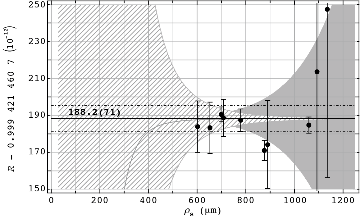
Figure 5-10: Summary of all our data for R vs \rho_s for ^{13}\text{C}_2\text{H}_2^+ / ^{14}\text{N}_2^+ . Each point is the result of an interpolation of the data at V_{\text{gr}}^{\text{t}} = V_{\text{gr}}^{\text{optct}} (see Fig. 5-8). Also shown are the uncertainty bands from our imperfect knowledge of the trapping field parameters (right) and the cyclotron radii imbalance (left). The final value for the measured R is represented by a solid horizontal line with the 1\sigma confidence interval denoted by the dashed line. The offset that was subtracted from every point is approximately the frequency difference predicted from the current mass table [20])
