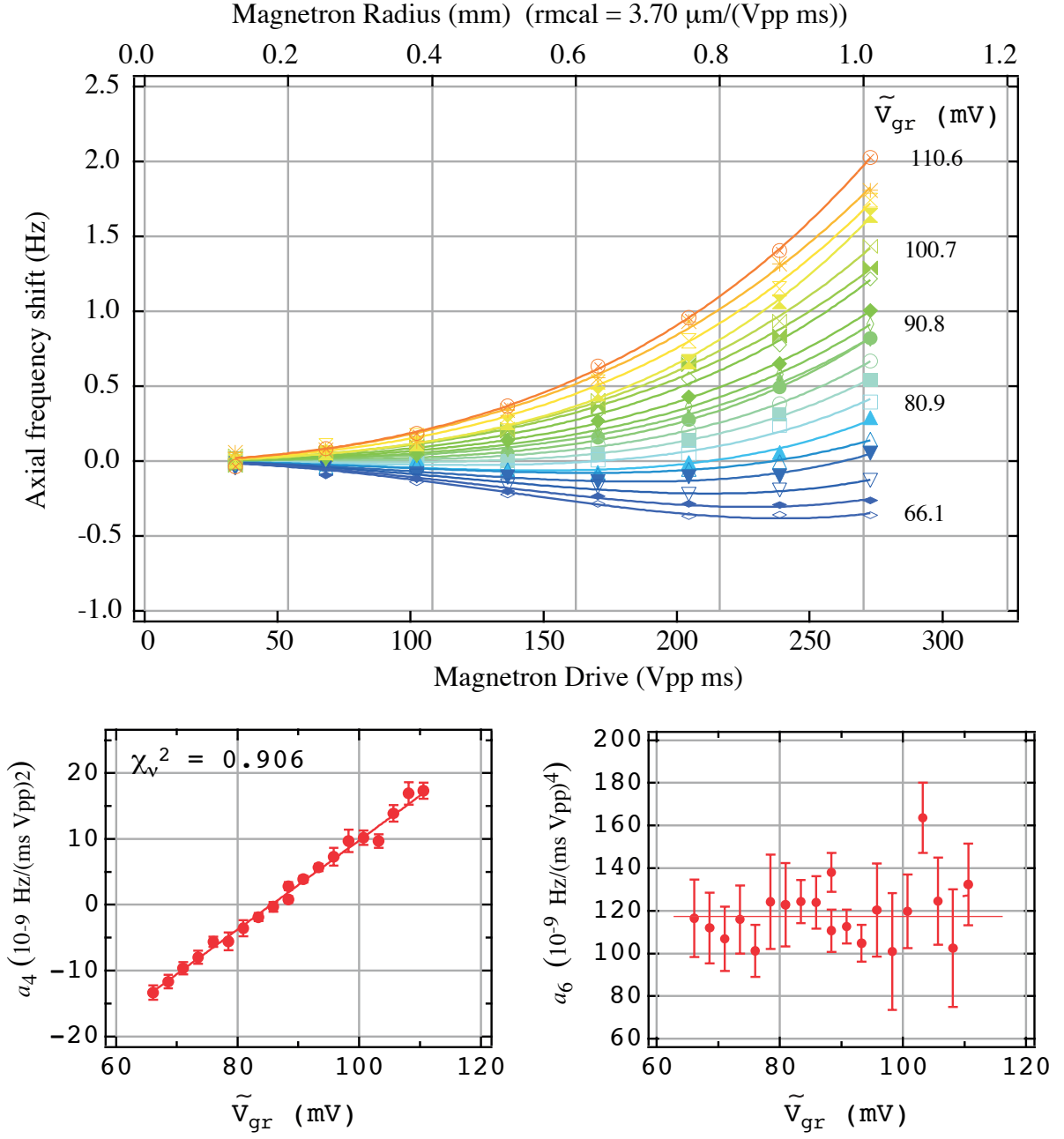
Figure 2-5: Typical “ f_z vs \rho_m ” data set obtained by measuring the axial frequency vs \rho_m vs \tilde{V}_{\text{gr}} with small axial pulses ( z \leq 200 \mu\text{m} ). Each curve of \Delta f_z vs \rho_m is fit with a polynomial of the form \Delta f_z = a_4 \rho_m^2 + a_6 \rho_m^4 .
