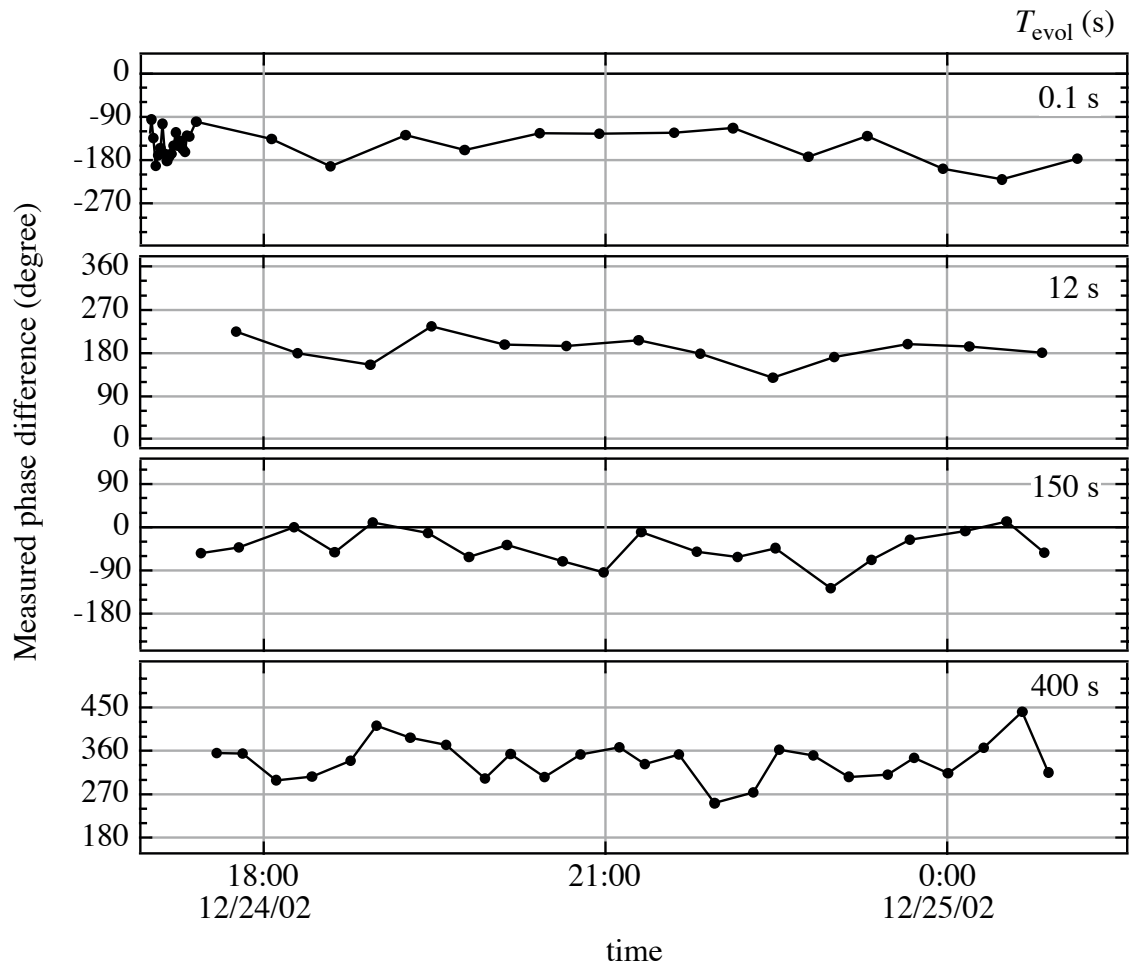
Figure 4-2: The raw data from a data set: the cyclotron phase differences (modulo 360^\circ ) accumulated after various T_{\text{evol}} as a function of time.
