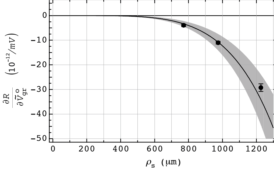
Figure 6-2: Measured slope \partial R/\partial V_{\text{gr}}^t using \text{H}^{32}\text{S}^+/\text{H}^{33}\text{S}^+ compared to the expected slope from our independent measurements of the trap field imperfections (and uncertainty). V_{\text{gr}}^t is related to the voltage applied to one of the electrodes of our trap (guard ring) which affects C_4 . These results show that we understand the effect of field imperfections on our measured ratio.
