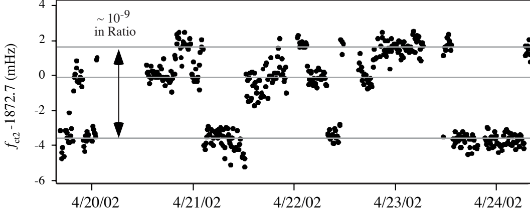
Figure 3-4: The measured (trap) cyclotron frequency difference \omega_{\text{ct2}} vs time for ^{14}\text{N}_2^+/\text{CO}^+ . The data exhibit abrupt and very large jumps between a few discrete values. Note that these jumps occurred on average every 8 hours, which made them very painful to study (this data set spans over 100 hours of data !). After over one year of investigation, we found that these correspond to black-body induced quantum jumps between the first few rotational states of the \text{CO}^+ molecule.
