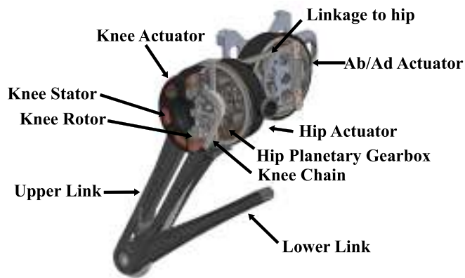
Fig. 2: Cheetah 3 Leg Design. One leg showing the 3 actuators, with a cutaway view of the knee actuator.
