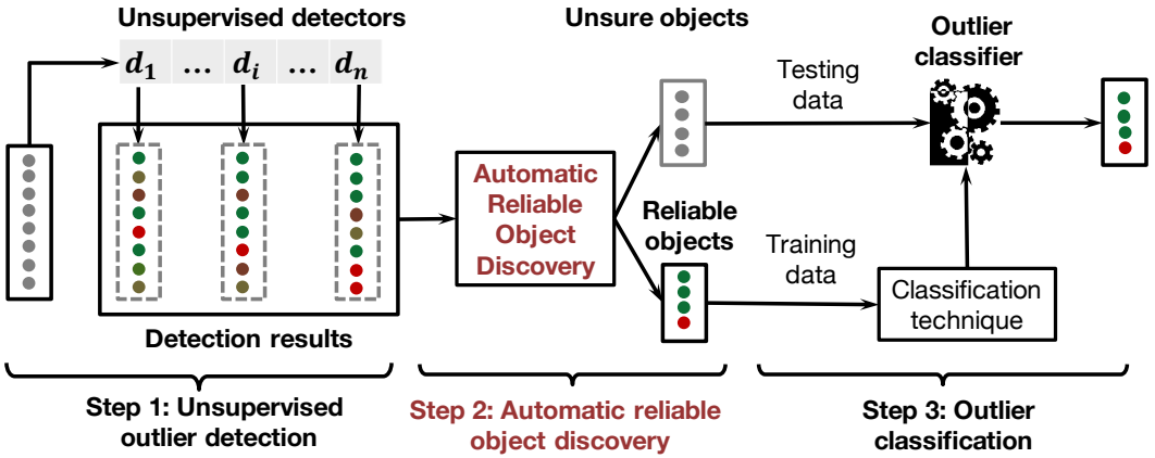
Fig. 1. AutoOD Framework
