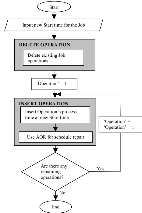
Fig. 4. Urgent Job
