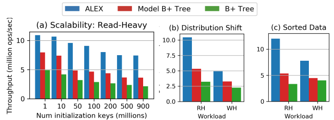
Figure 12: ALEX maintains high throughput when scaling to large datasets and under data distribution shifts. (RH = Read-Heavy, WH = Write-Heavy)
