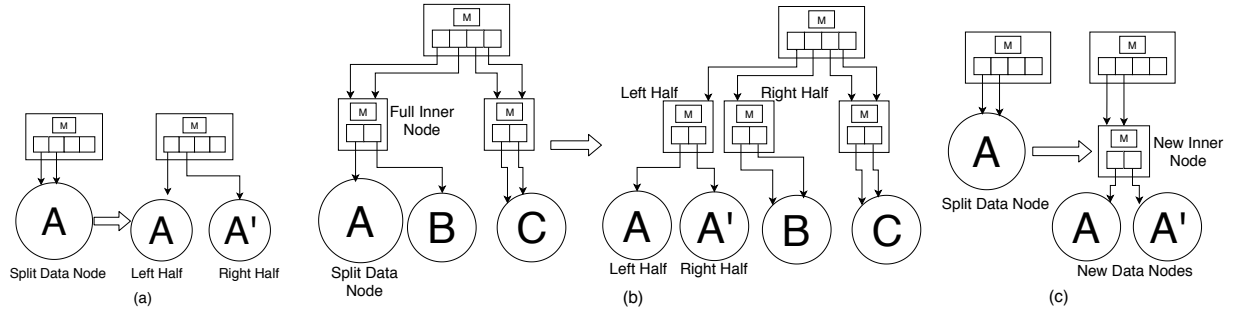
Figure 5: Node Splits
