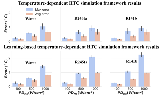
Fig. 6: Non-uniform power profile maximum and average temperature error validation results. \dot{P}D_{Hs} stands for hot spot power density. The accuracy results for non-uniform validation tests are shown in Fig. 6. Compared to the COMSOL model, the temperature-dependent HTC simulation framework has a maximum error of 1.34^\circ\text{C} with an average speedup of 22\times . The maximum error and average error of our proposed learning-based temperature-dependent HTC simulation framework are 2.59^\circ\text{C} and 0.98^\circ\text{C} , respectively and the average speedup is 21\times . Note that the accuracy results include all of the validation floorplans and geometries. Since we replace temperature-dependent HTC correlation lookup table with machine learning regression models, the simulation speedup and accuracy are expected to decrease. However, our proposed model still achieves good accuracy and speedup when compared to the COMSOL model. Most importantly, our proposed learning-based temperature-dependent HTC simulation framework enables accurate thermal simulations with valid and comprehensive geometries.
