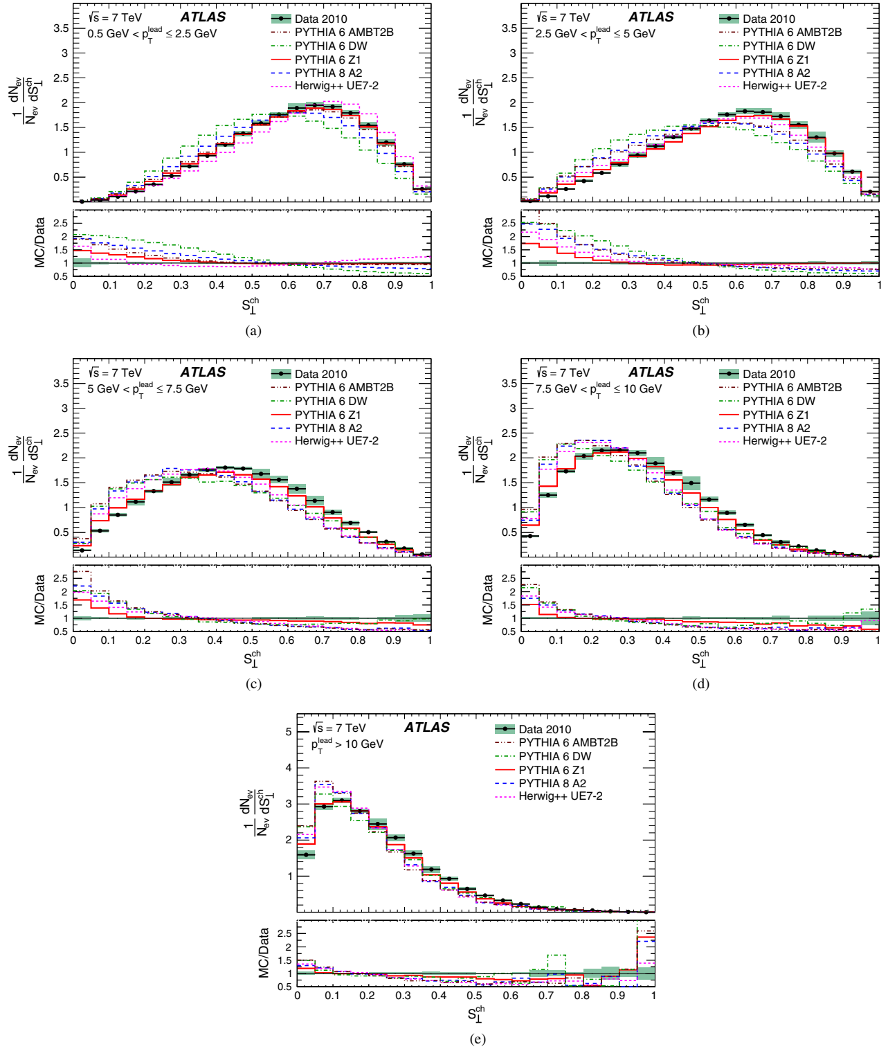
FIG. 5 (color online). Normalized distributions of transverse sphericity using at least six charged particles with p_T > 0.5 \text{ GeV} and |\eta| < 2.5 for different requirements on the transverse momentum of the leading charged-particle, p_T^{\text{lead}} . The error bars show the statistical uncertainty while the shaded area shows the combined statistical and systematic uncertainty. Where not visible, the statistical error is smaller than the marker size.
