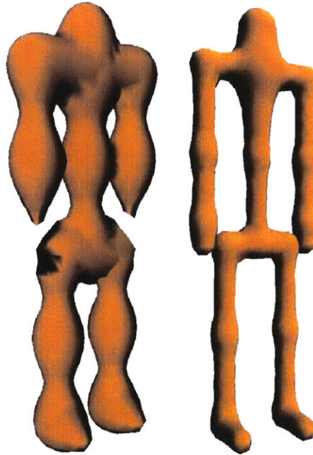
Figure 5-3: The biped before and after IMPS' implicit function reformulation. The figure on the left is rendered using IMPS' Marching Cubes implementation, while the figure on the right is triangulated using Tesselator3MP .
