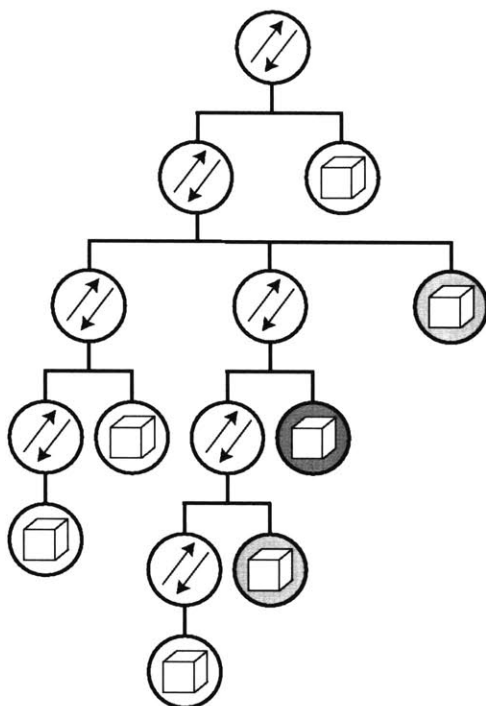
Figure 3-1: Blending rules IMPS imposes upon a hierarchy of Transforms and Shapes. Points belonging to the dark gray Shape node add in contributions from the light gray nodes, which correspond to its parents and children.
