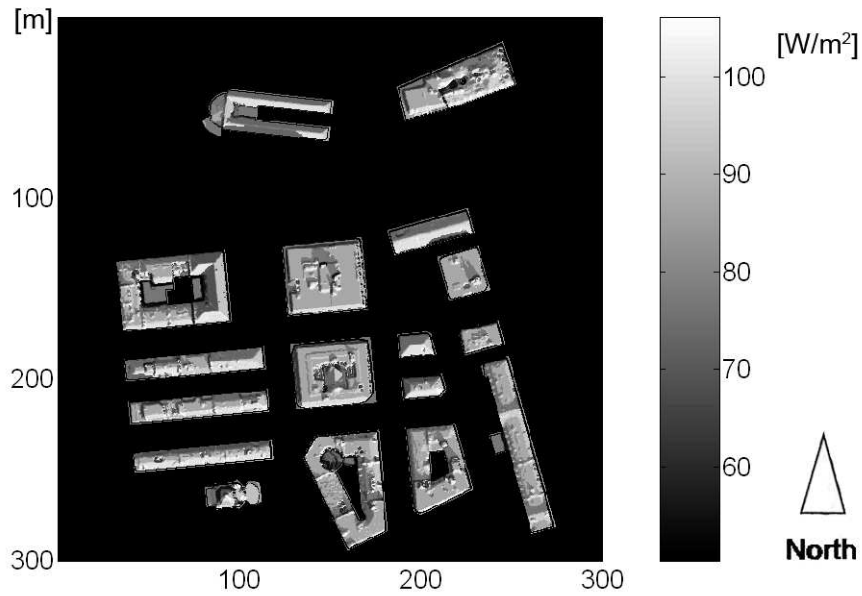
Fig. 10. Top view with irradiance values (in \text{W}/\text{m}^2 ) on roofs at 10 AM in the morning on December 10
