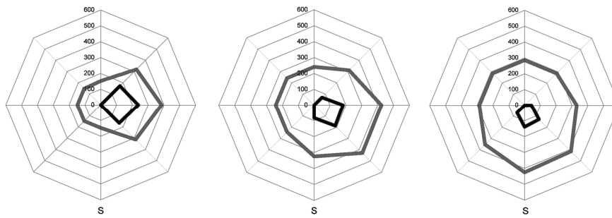
Fig. 11. Polar plots of solar irradiances on vertical surfaces for Geneva on the average day of June; in black beam radiation, in dark gray diffuse radiation (values are expressed in \text{W}/\text{m}^2 ). From left: irradiances at (a) 8 AM, (b) 10 AM, (c) 12 PM
