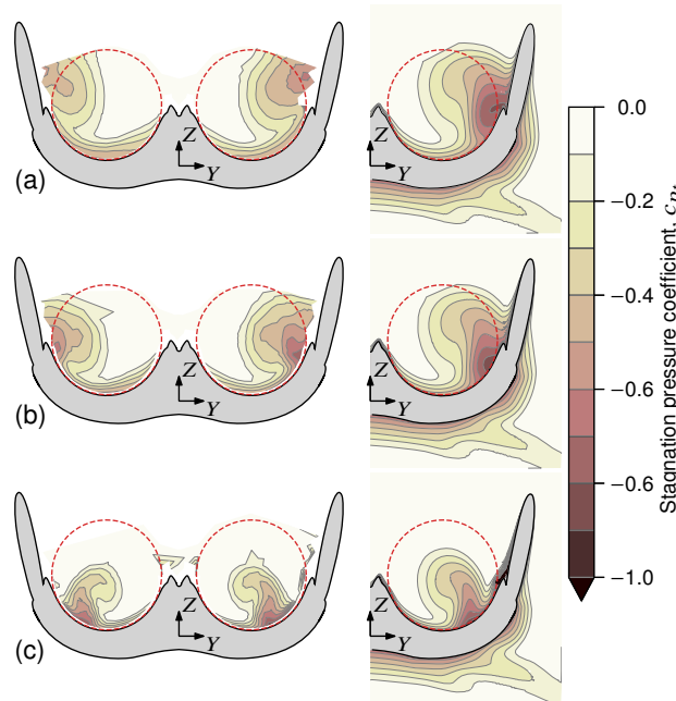
Fig. 14 Effect of propulsor power level on inlet stagnation pressure distortion: measured (left) and computed (right) inlet stagnation pressure coefficient at \alpha = 8^\circ ; (a) low power, (b) cruise power, and (c) high power
