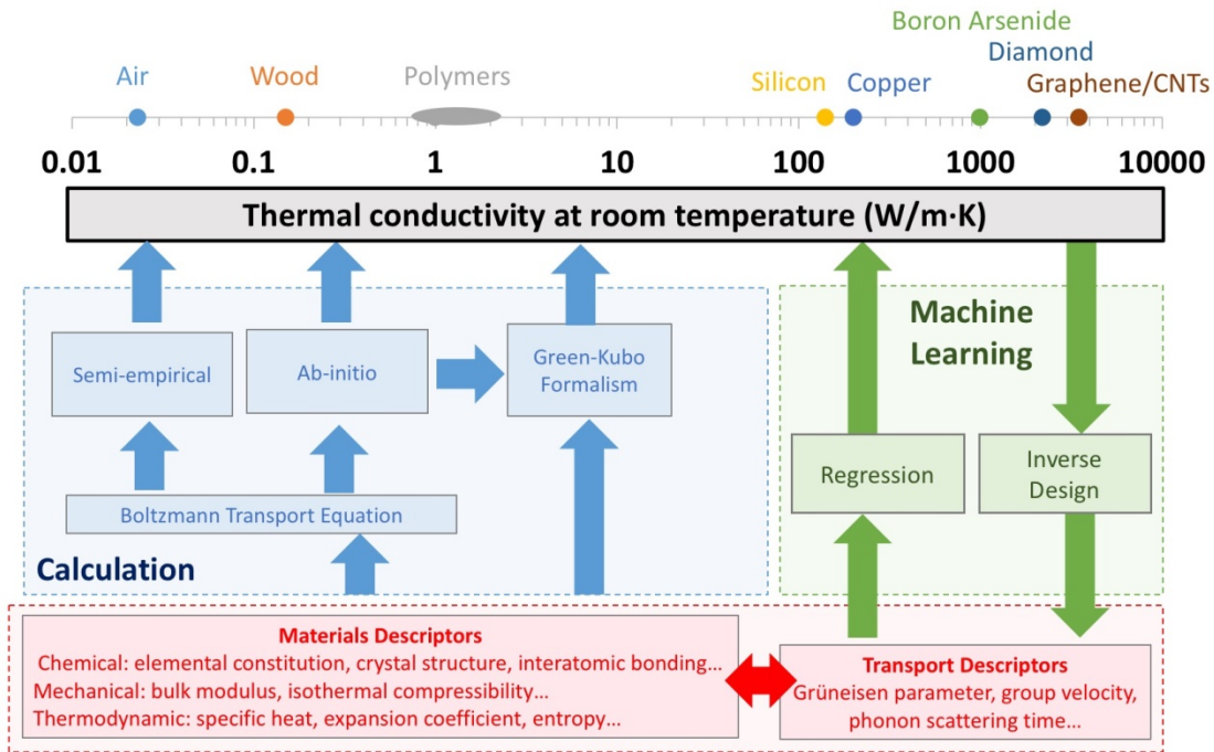
Fig. 1. The range of thermal conductivity can span more than six orders of magnitude. Obtaining accurate values of thermal conductivity and understanding the physical reason for the thermal conductivity is a challenge as calculations are computationally expensive and is typically a one-directional model-based approach of tweaking and observing. With machine learning, the cycle of materials discovery is now complete where we can correlate thermal conductivity with descriptors, providing the feedback to speed up materials innovation and discovery.
