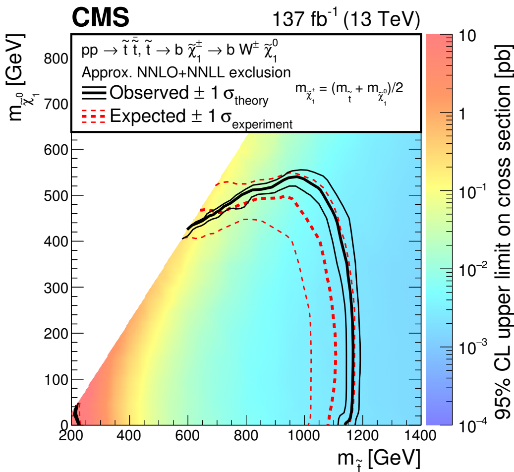
Figure 7. Exclusion limits at 95% CL for the pp \rightarrow \tilde{t} \tilde{t}^* \rightarrow b \bar{b} \tilde{\chi}_1^+ \tilde{\chi}_1^- (\tilde{\chi}_1^+ \rightarrow W \tilde{\chi}_1^0) scenario. The mass of \tilde{\chi}_1^\pm is chosen to be (m_{\tilde{t}} + m_{\tilde{\chi}_1^0})/2 . The colored map illustrates the 95% CL upper limits on the product of the production cross section and branching fraction. The area enclosed by the thick black curve represents the observed exclusion region, and that enclosed by the thick, dashed red curve represents the expected exclusion. The thin dotted (red) curves indicate the region containing 68% of the distribution of limits expected under the background-only hypothesis. The thin solid (black) curves show the change in the observed limit by varying the signal cross sections within their theoretical uncertainties.
