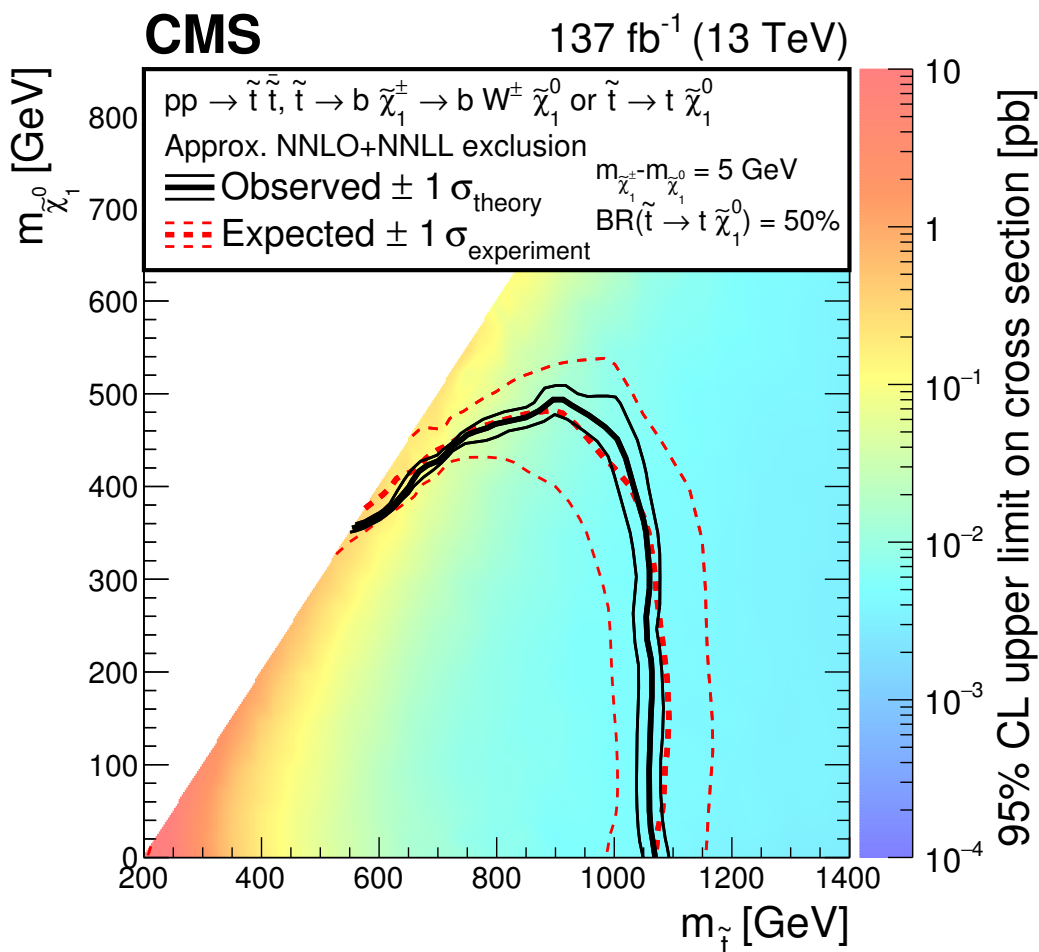
Figure 8. Exclusion limits at 95% CL for the pp \rightarrow \tilde{t}\tilde{t} \rightarrow t b \tilde{\chi}_1^+ \tilde{\chi}_1^0 (\tilde{\chi}_1^+ \rightarrow W^* \tilde{\chi}_1^0) scenario. The mass difference between the \tilde{\chi}_1^\pm and the \tilde{\chi}_1^0 is taken to be 5 GeV. The colored map illustrates the 95% CL upper limits on the product of the production cross section and branching fraction. The area enclosed by the thick black curve represents the observed exclusion region, and that enclosed by the thick, dashed red curve represents the expected exclusion. The thin dotted (red) curves indicate the region containing 68% of the distribution of limits expected under the background-only hypothesis. The thin solid (black) curves show the change in the observed limit by varying the signal cross sections within their theoretical uncertainties.
