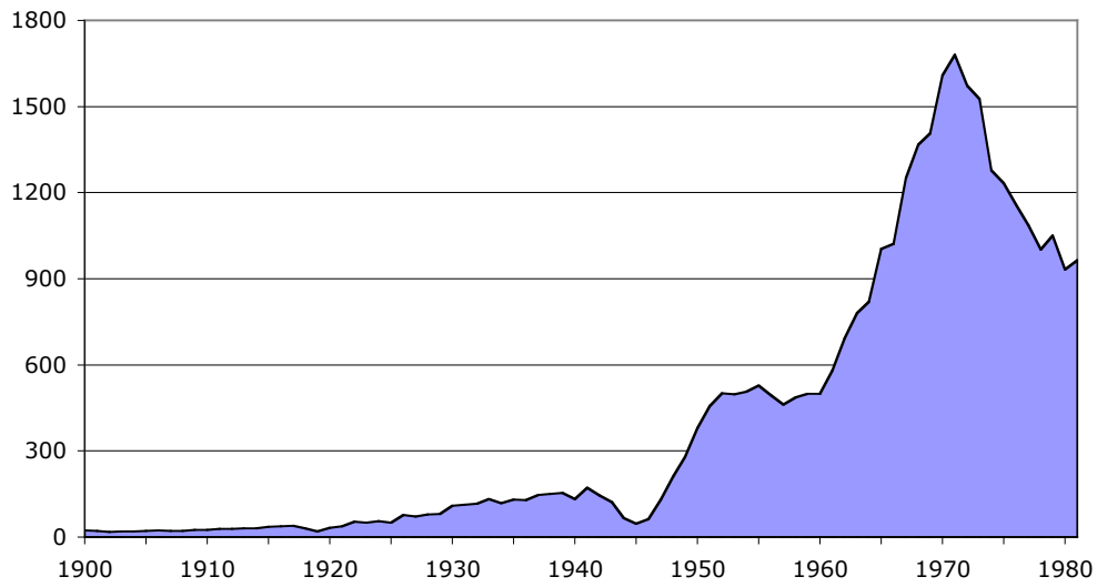
Figure 5. Number of physics Ph.D.s granted per year in the United States, 1900-81.
