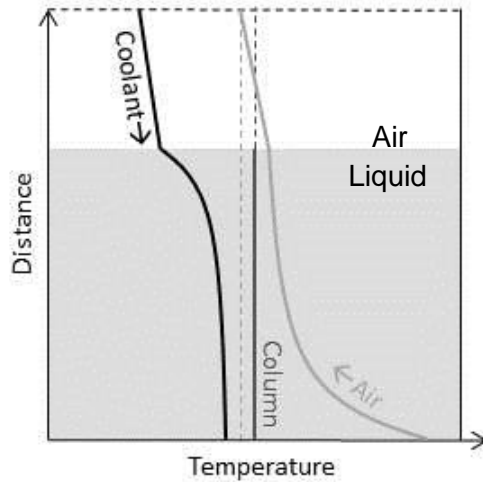
Figure 6: Coolant and moist air stream temperature profiles in a column showing the air leaving below the column liquid temperature.
