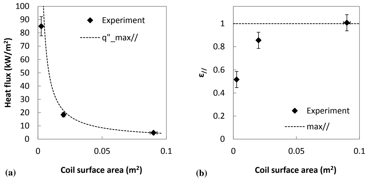
Figure 3: Effect of coil area on (a) heat flux and (b) effectiveness.
