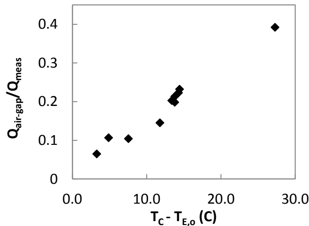
Figure 7: The fraction of heat transfer occurring in air gap increases with the liquid-side temperature pinch.
