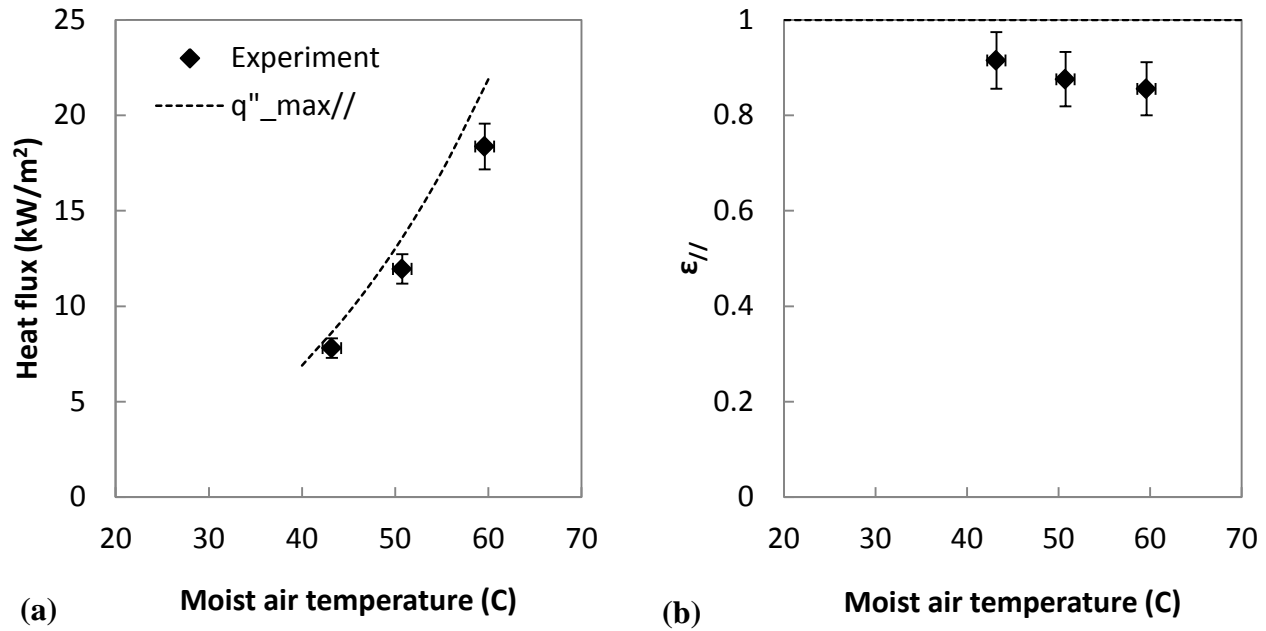
Figure 4: Effect of moist air temperature on (a) heat flux and (b) effectiveness.
