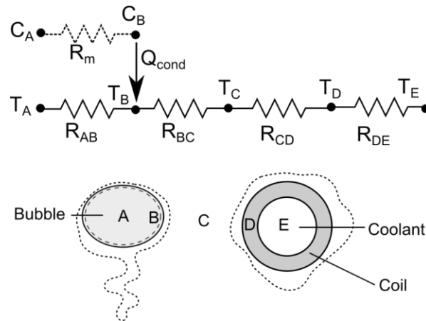
Figure 2: Resistance network from [12] governing heat and mass transfer in the liquid region of a bubble column dehumidifier, with resistances ( R ), mean concentrations ( C ) and mean temperatures ( T ). Node B is just inside the bubble surface. C_B is a saturated state at T_B .
