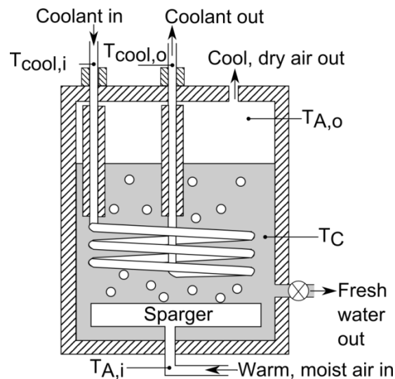
Figure 1: Schematic diagram of the experimental dehumidifier.
