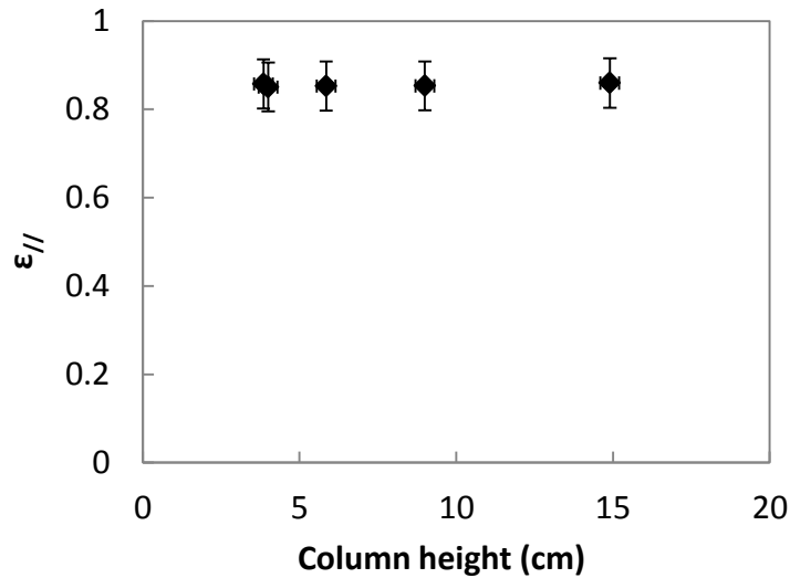
Figure 5: Effectiveness of varying column heights, showing that the critical height is below the minimum height necessary to cover the coil.
