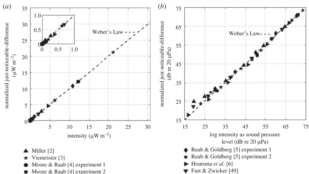
Figure 2. Just-noticeable-differences in acoustic intensity approximately follow Weber's Law. (a) Just-noticeable-differences as a function of acoustic intensity stimulus from artificial sound sources obtained from decades of psychophysical experiments measuring human response to sound with broad spectra filling the entire 128 Hz critical band centred at 1000 Hz [2–6,49]. Just-noticeable-differences from each independent experiment display excellent fit to a straight line and consequently Weber's Law. The independent experiments employed acoustic signal stimuli of differing duration and different human subjects which lead to best-fit lines with differing slopes across experiments. Best-fit slopes are normalized to the same value to visually compare linearity of just-noticeable-differences versus stimulating intensity across experiments (electronic supplementary material, table S1). Data shown roughly 10 dB above absolute lowest detectable sound pressure level to avoid contamination from auditory system self-noise or ambient noise contamination. Inset image zooms in on lower intensities. (b) Same values as plotted in (a) but in decibels as a function of stimulating sound pressure level.
