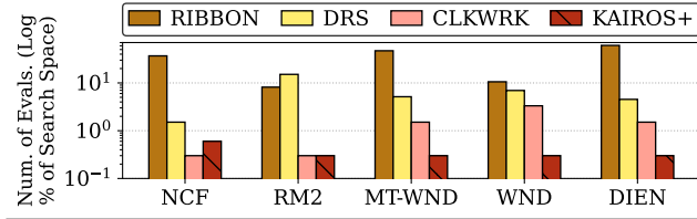
Figure 10: KAIROS+ has low evaluation overhead.
