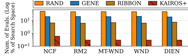
Figure 11: KAIROS+ versus competing search algorithms.
