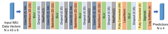
Figure 6: ViWatch Backbone Convolutional Neural Network Architecture.
